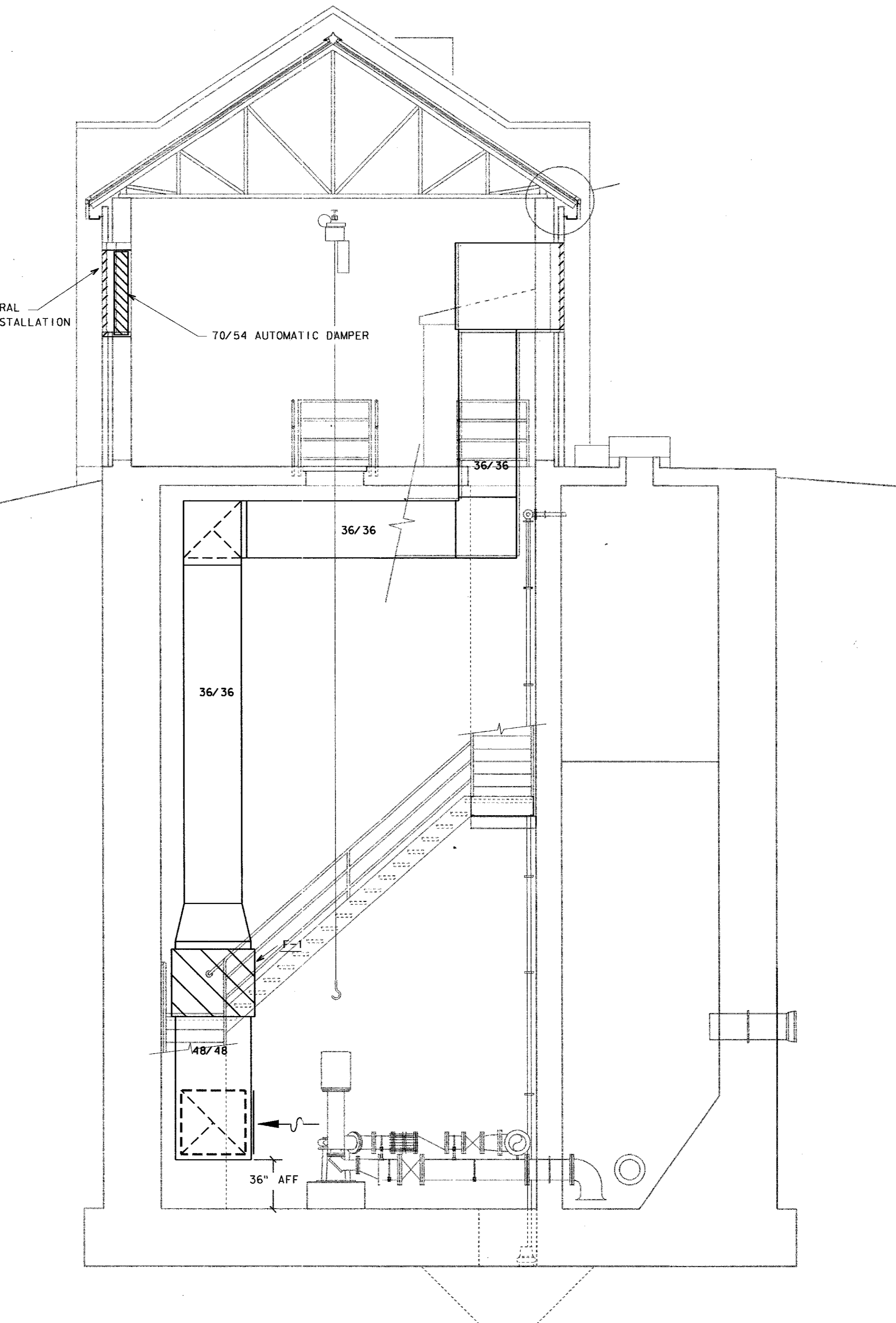
SECTION B 1/4" = 1'-0"
