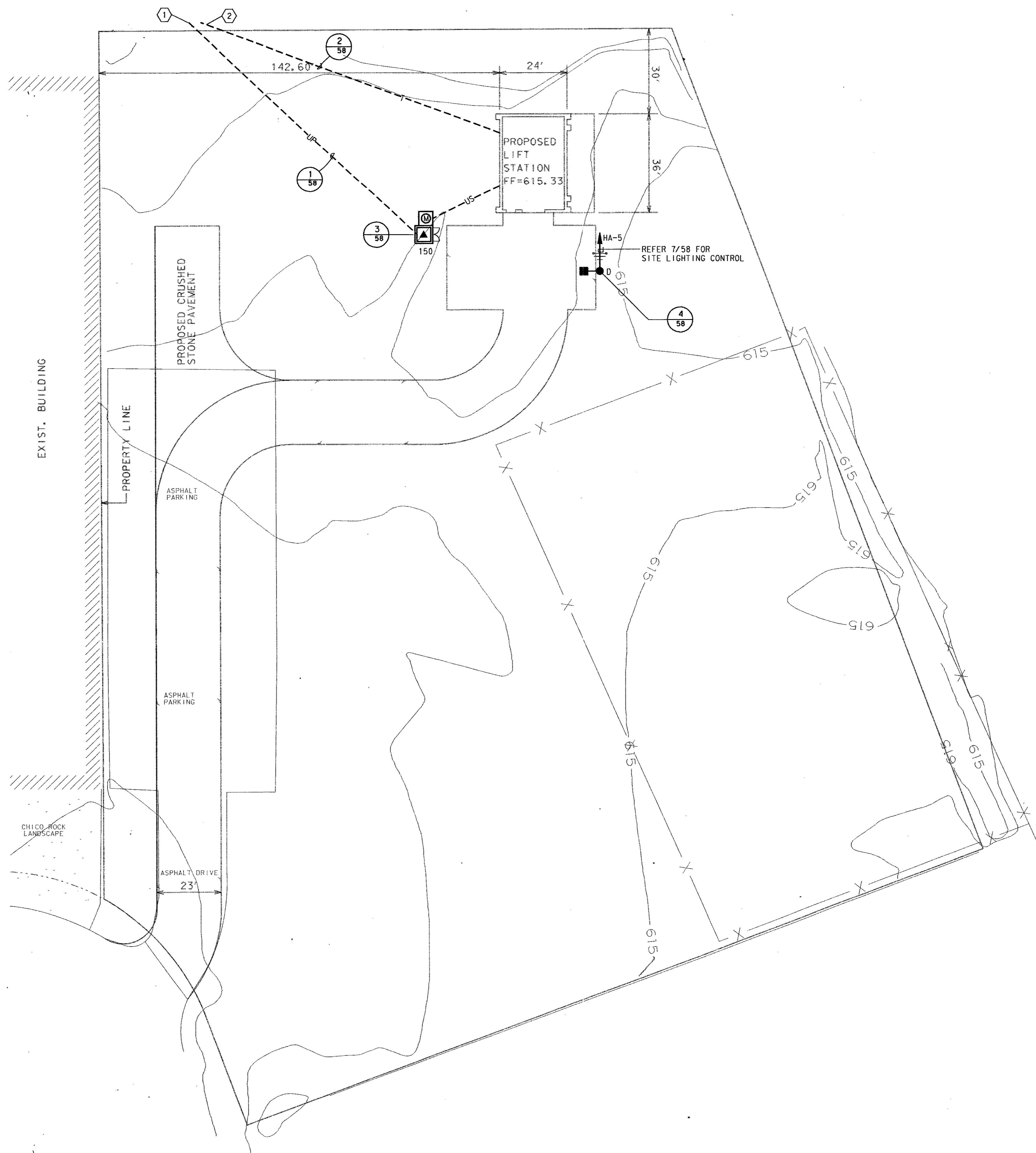
A SITE PLAN - ELECTRICAL 55 SCALE: 1"=20'
