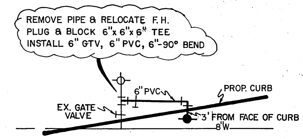
FH RELOCATION DETAIL
