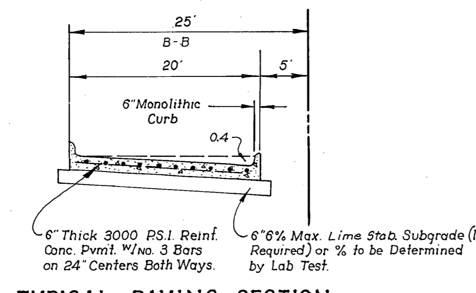
TYPICAL PAVING SECTION No Scale
