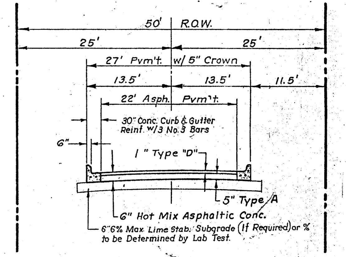
ALTERNATE PAVING SECTION No Scale
