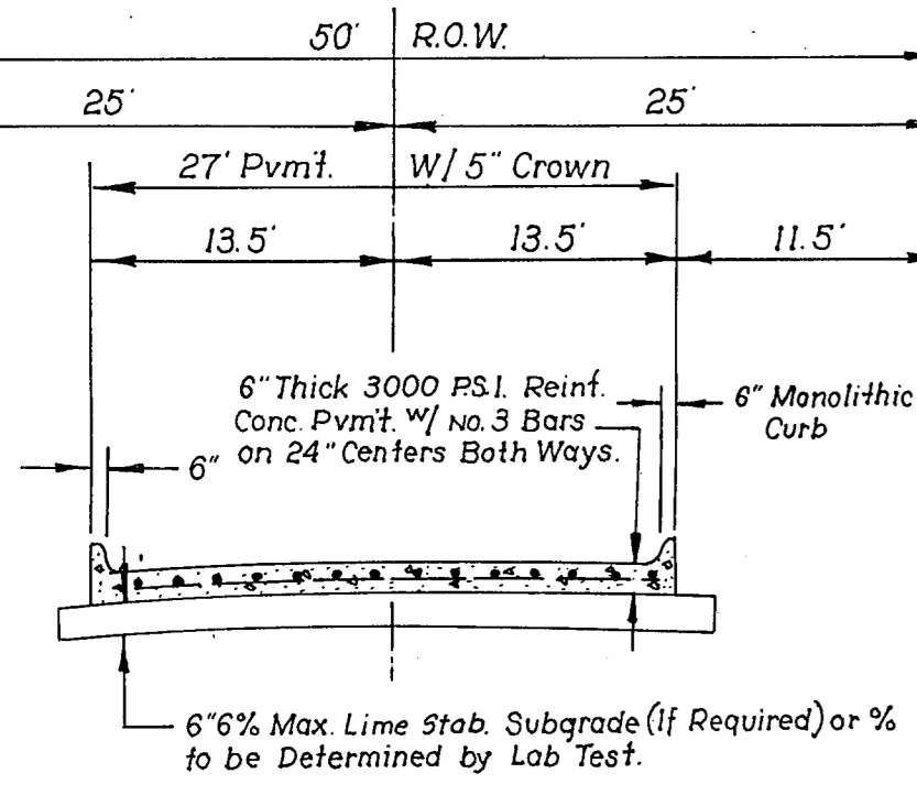
TYPICAL PAVING SECTION No Scale
