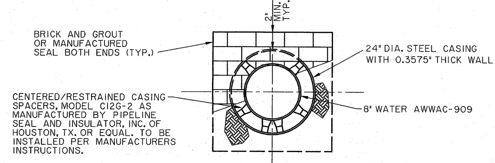
UNDERCROSSING BY OTHER THAN OPEN CUT N.T.S.
