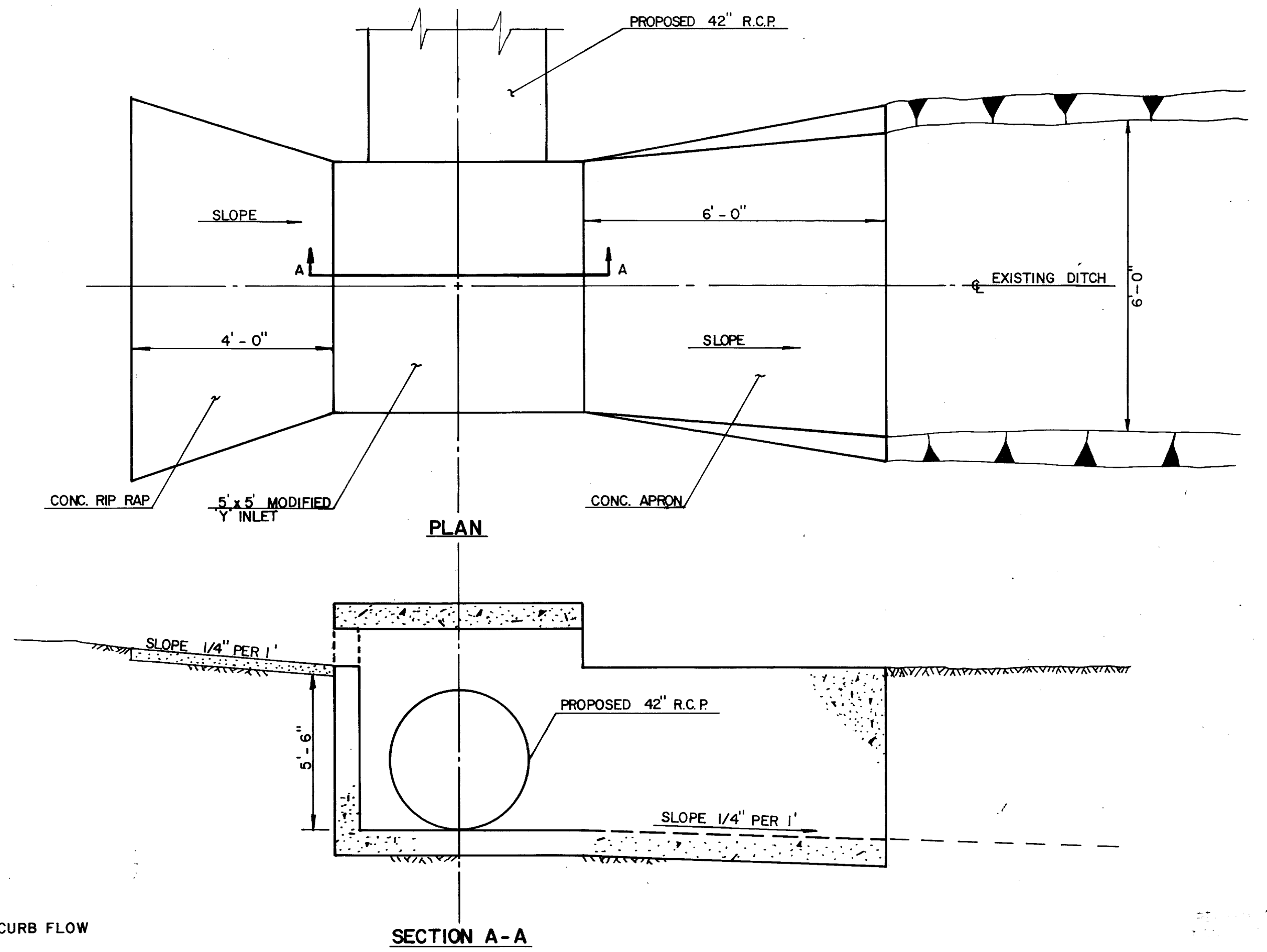
MODIFIED "Y" INLET SCALE: 1/2" = 1' SEE SHEET 11 LINE 'd'
