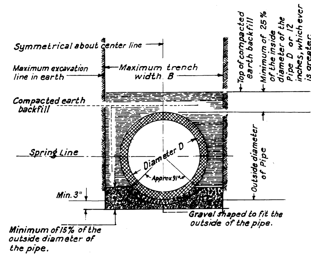
GRAVEL BEDDING
