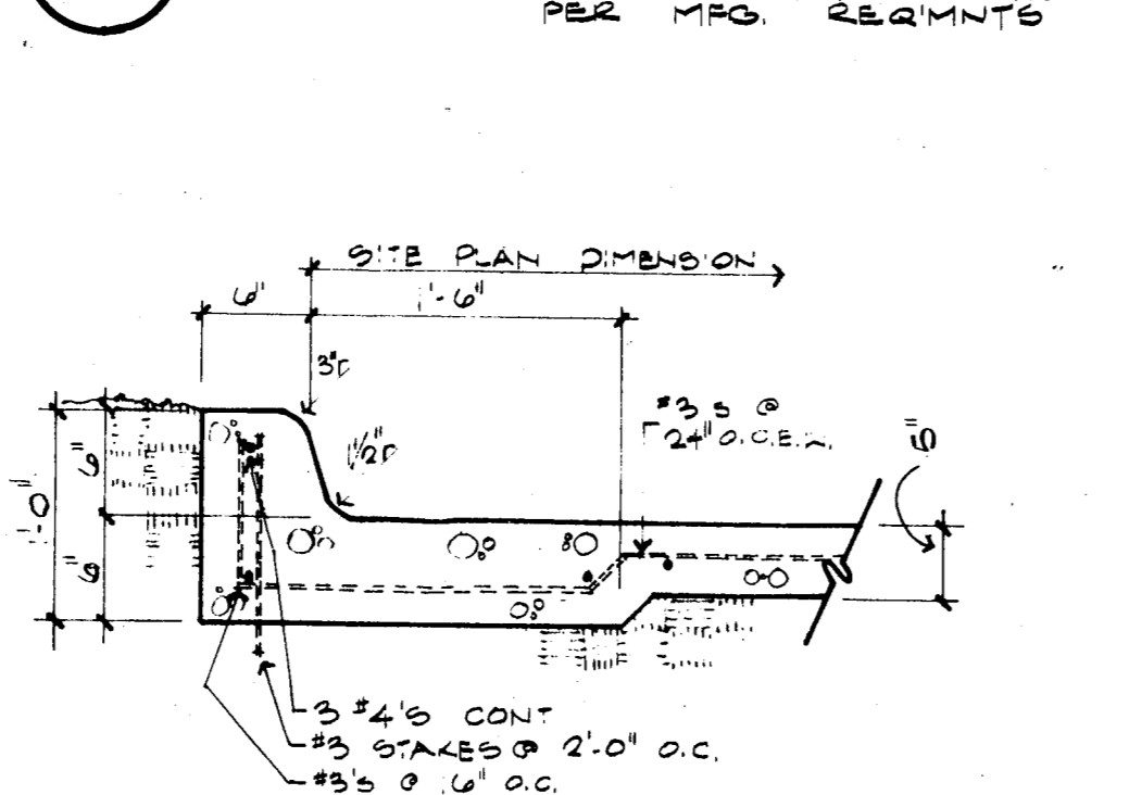
13 CONC. CURB SC: 1"=1'-0"
