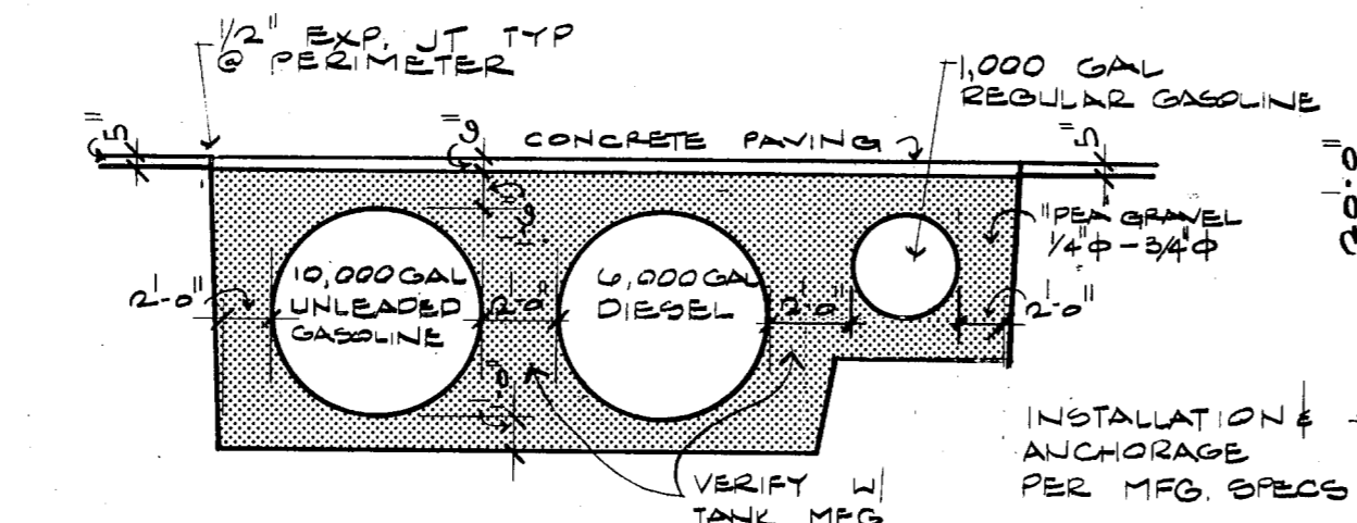
04 TANK SECTION SC: 1/8"=1'-0"
