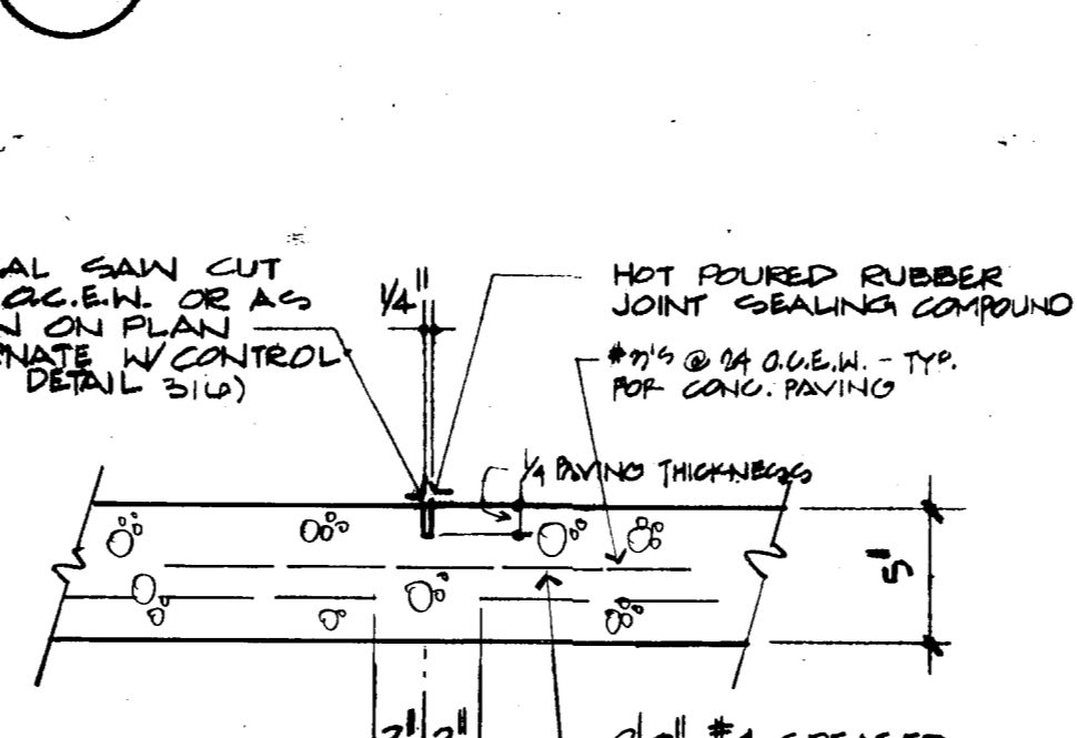
18 CONTRACTION JOINT SC: 1/2"=1'-0"
