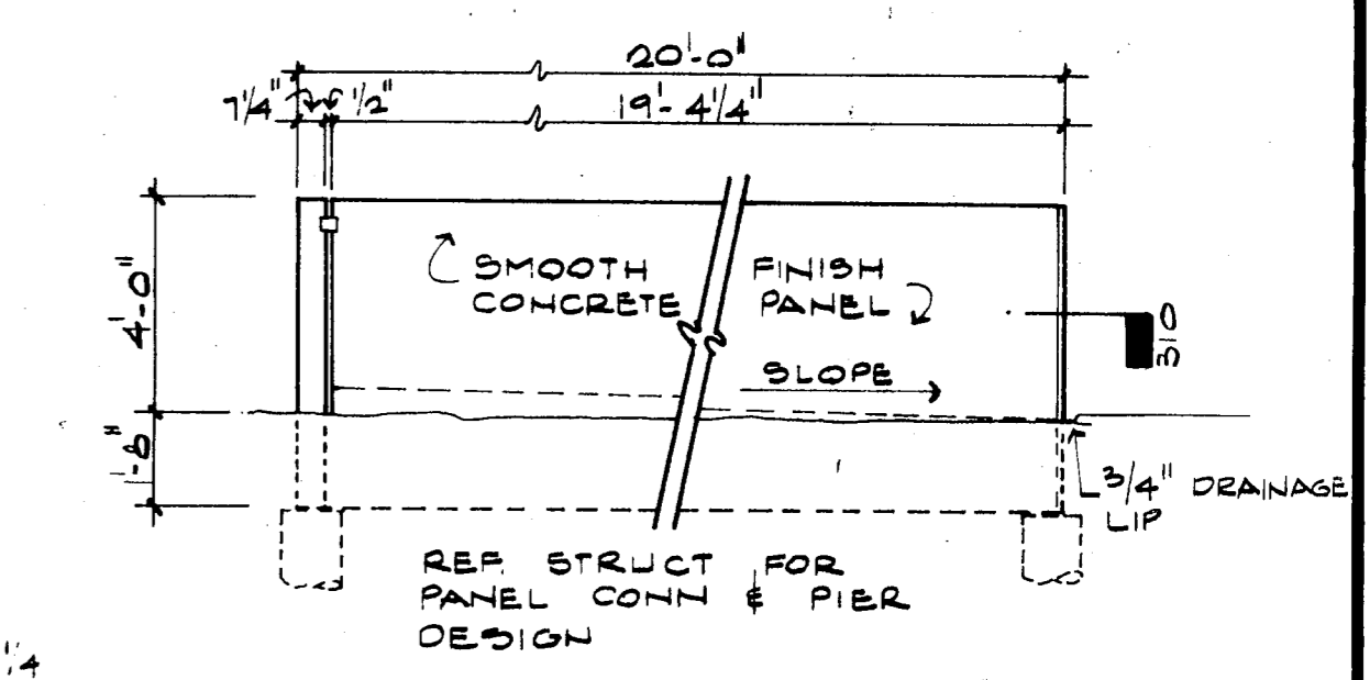
06 STORAGE AREA ELEVATION SC: 1/4"=1'-0"
