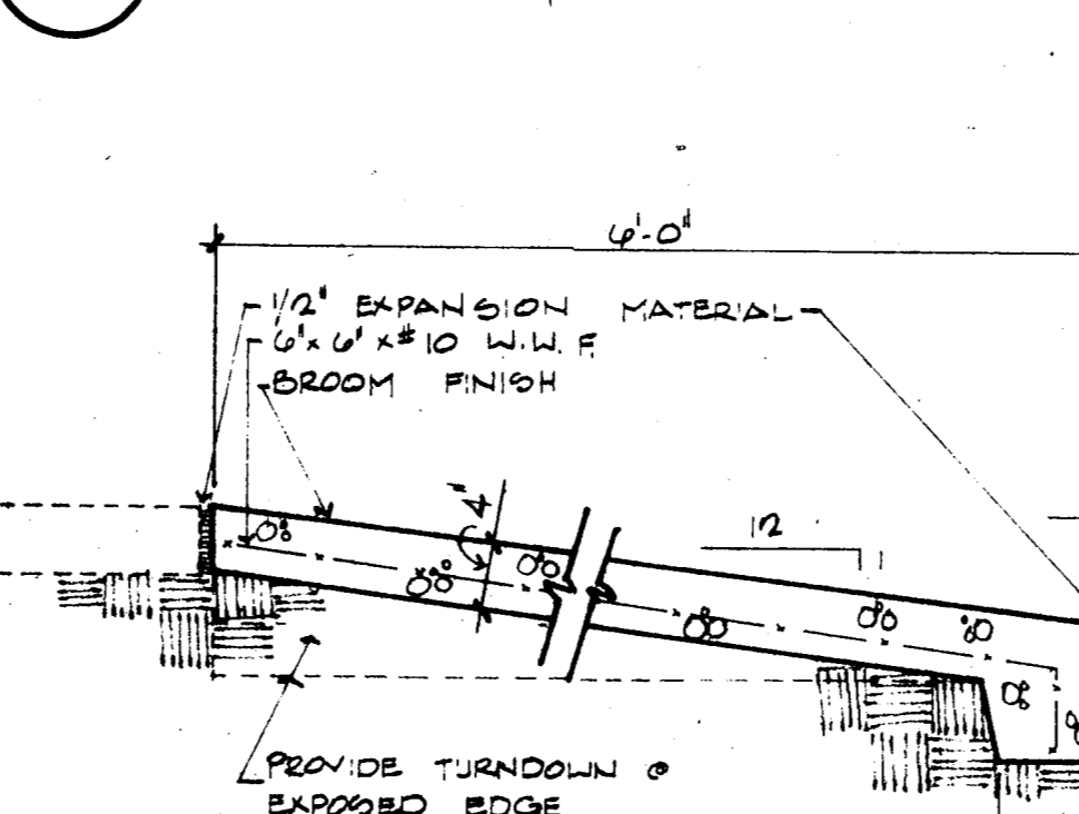
14 HANDICAP RAMP SC: 1"=1'-0"
