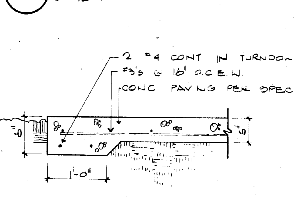
19 PAVING STOP SC: 1"=1'-0"
