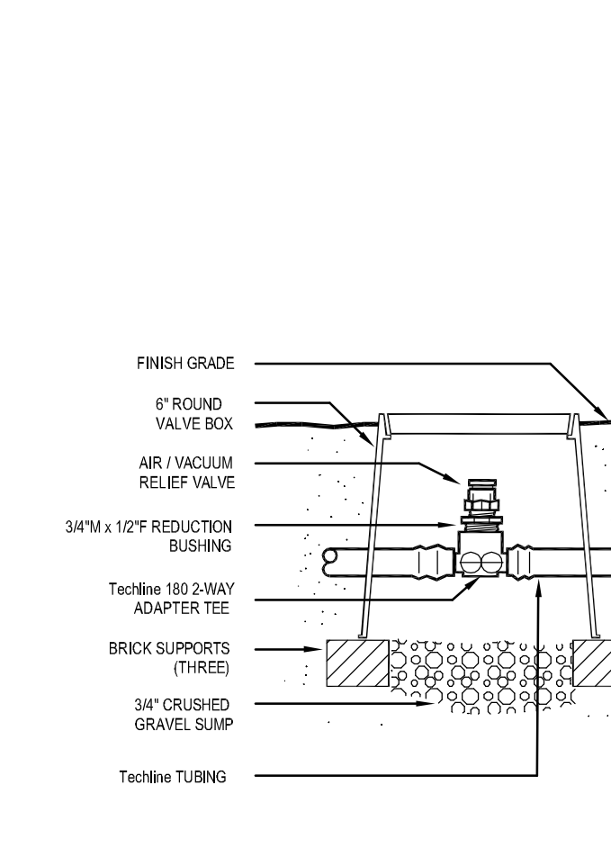
12 TechLine AIR/VACUUM RELIEF NOT TO SCALE
