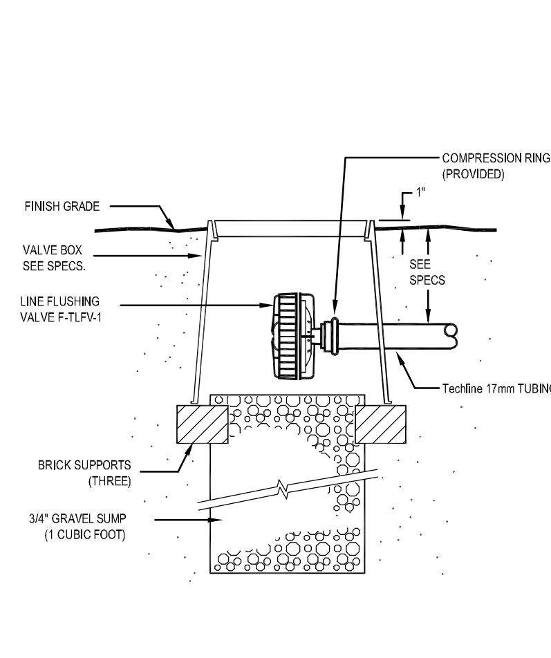
11 TechLine LINE FLUSHING VALVE NOT TO SCALE
