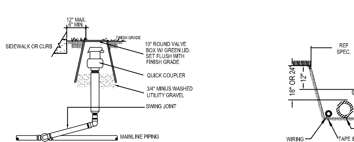
08 QUICK COUPLER NOT TO SCALE
