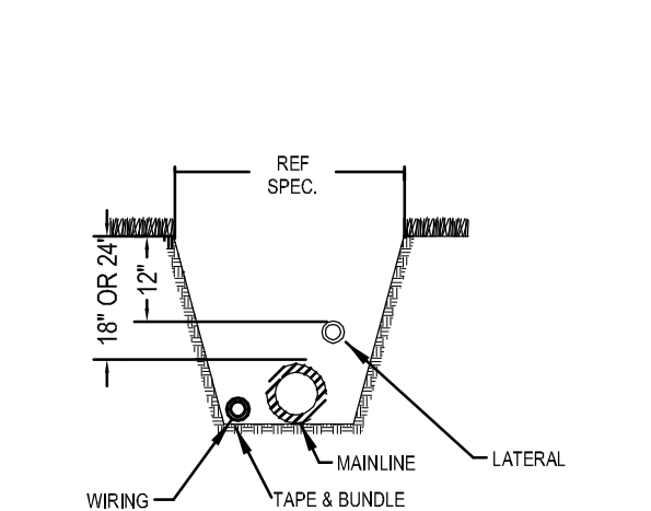
09 TRENCH DETAIL NOT TO SCALE
