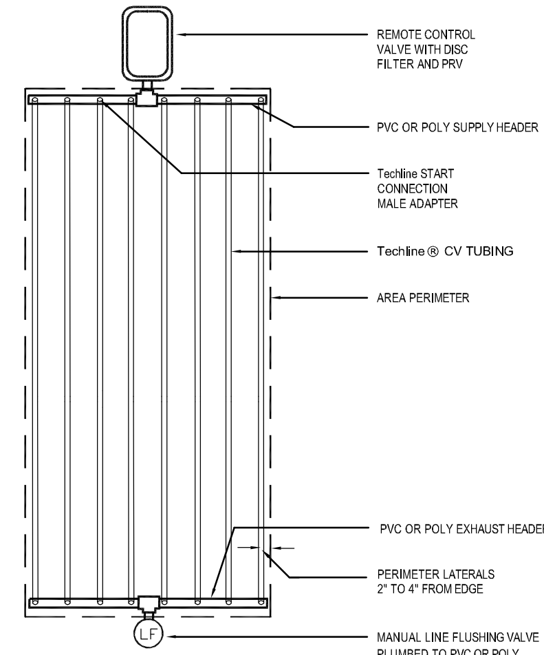
10 TechLine CV END FEED LAYOUT NOT TO SCALE
