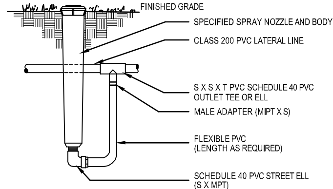
02 HIGH POP-UP SPRAY ASSEMBLY NOT TO SCALE
