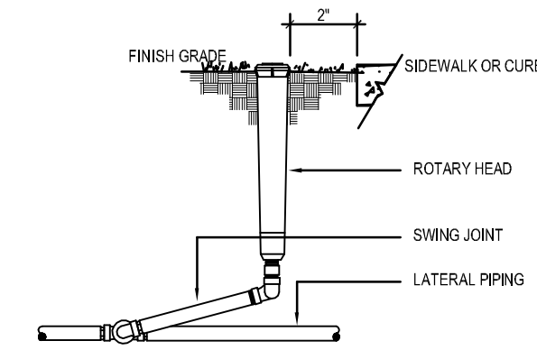
01 ROTARY HEAD NOT TO SCALE
