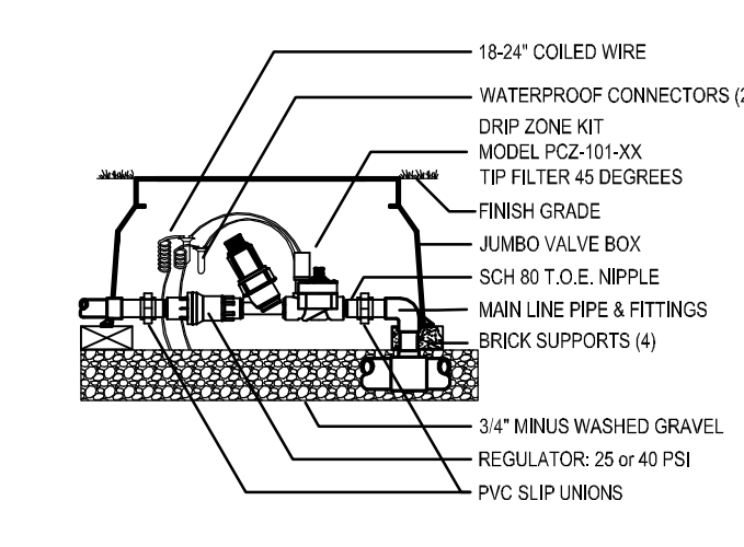
07 DRIP CONTROL VALVE NOT TO SCALE
