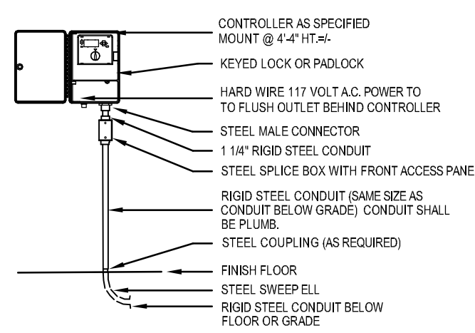
05 WALL MOUNTED CONTROLLER NOT TO SCALE
