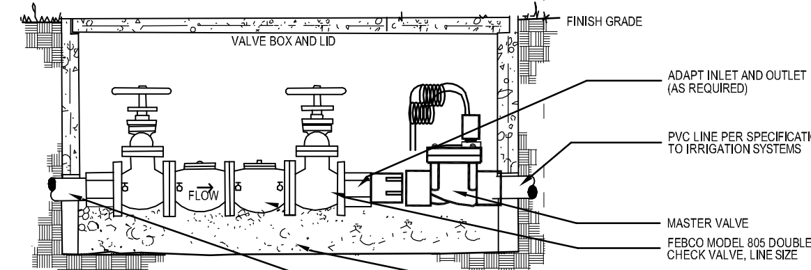
04 BACKFLOW PREVENTER NOT TO SCALE
