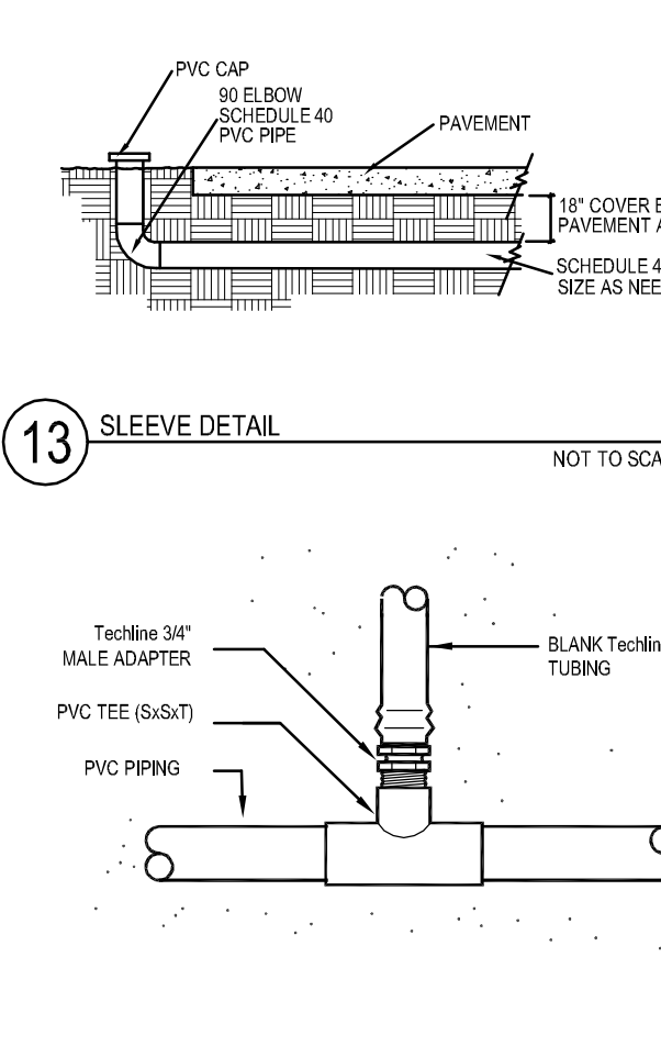
13 SLEEVE DETAIL NOT TO SCALE
