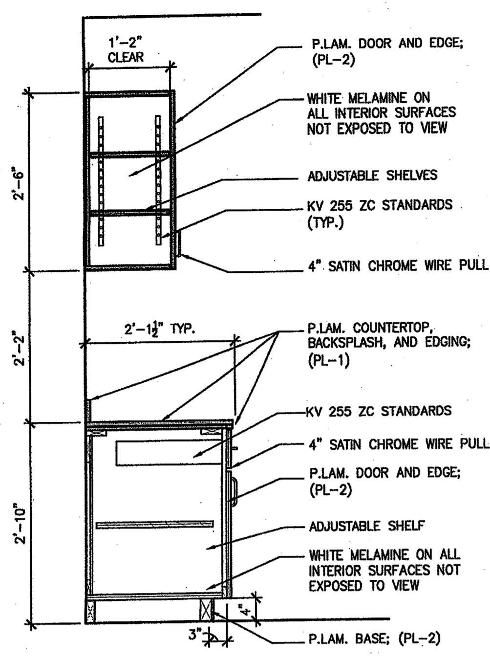
09 SECTION @ MILLWORK SCALE: 3/4" = 1'-0"
