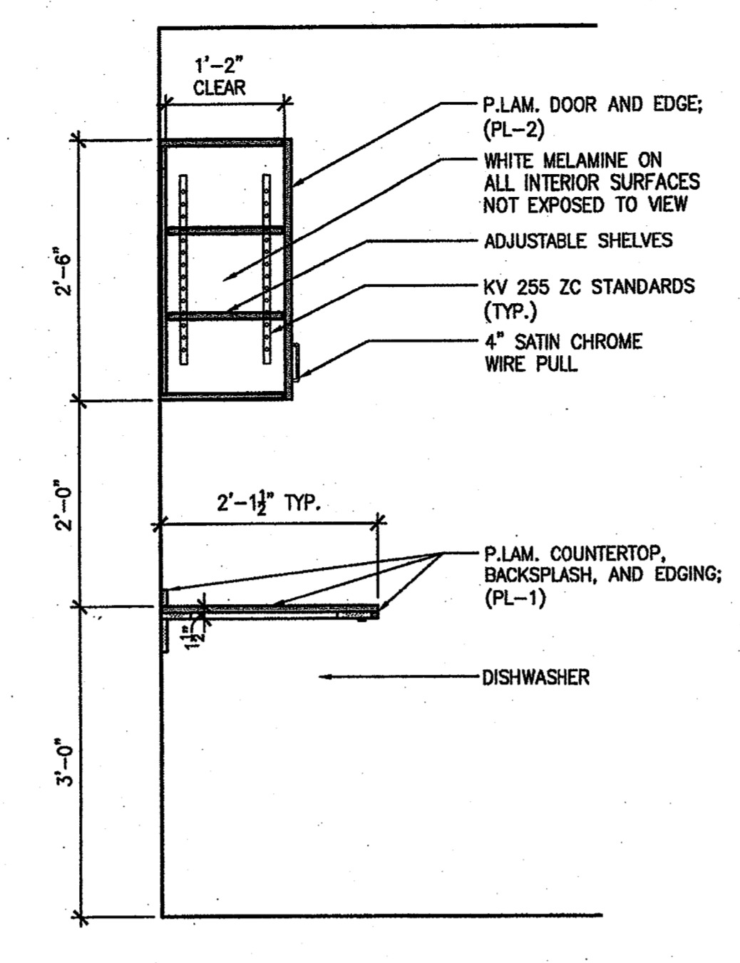
11 SECTION @ MILLWORK SCALE: 3/4" = 1'-0"
