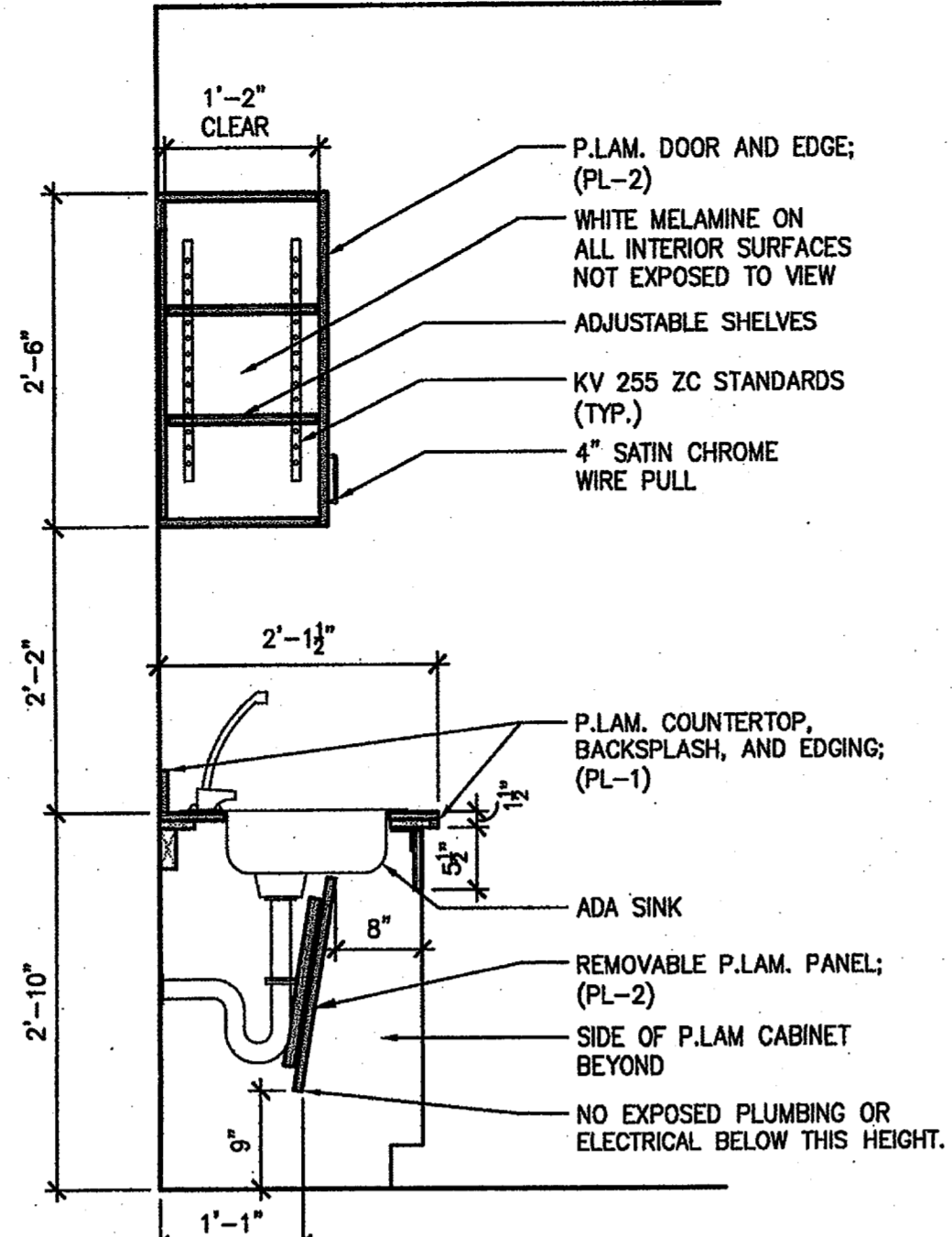
10 SECTION @ MILLWORK SCALE: 3/4" = 1'-0"
