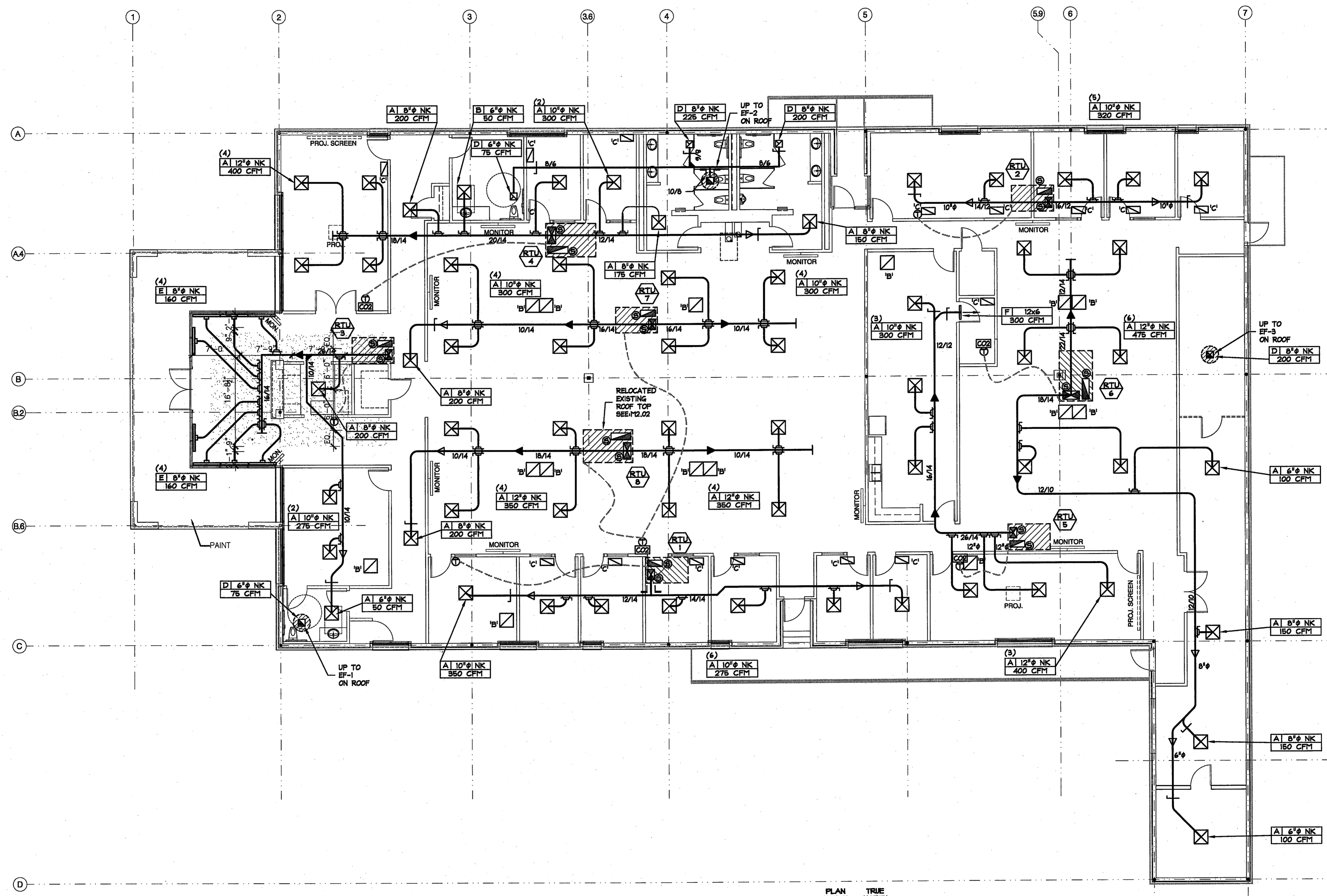
01 FLOOR PLAN - MECHANICAL SCALE: 1/8"=1'-0"
