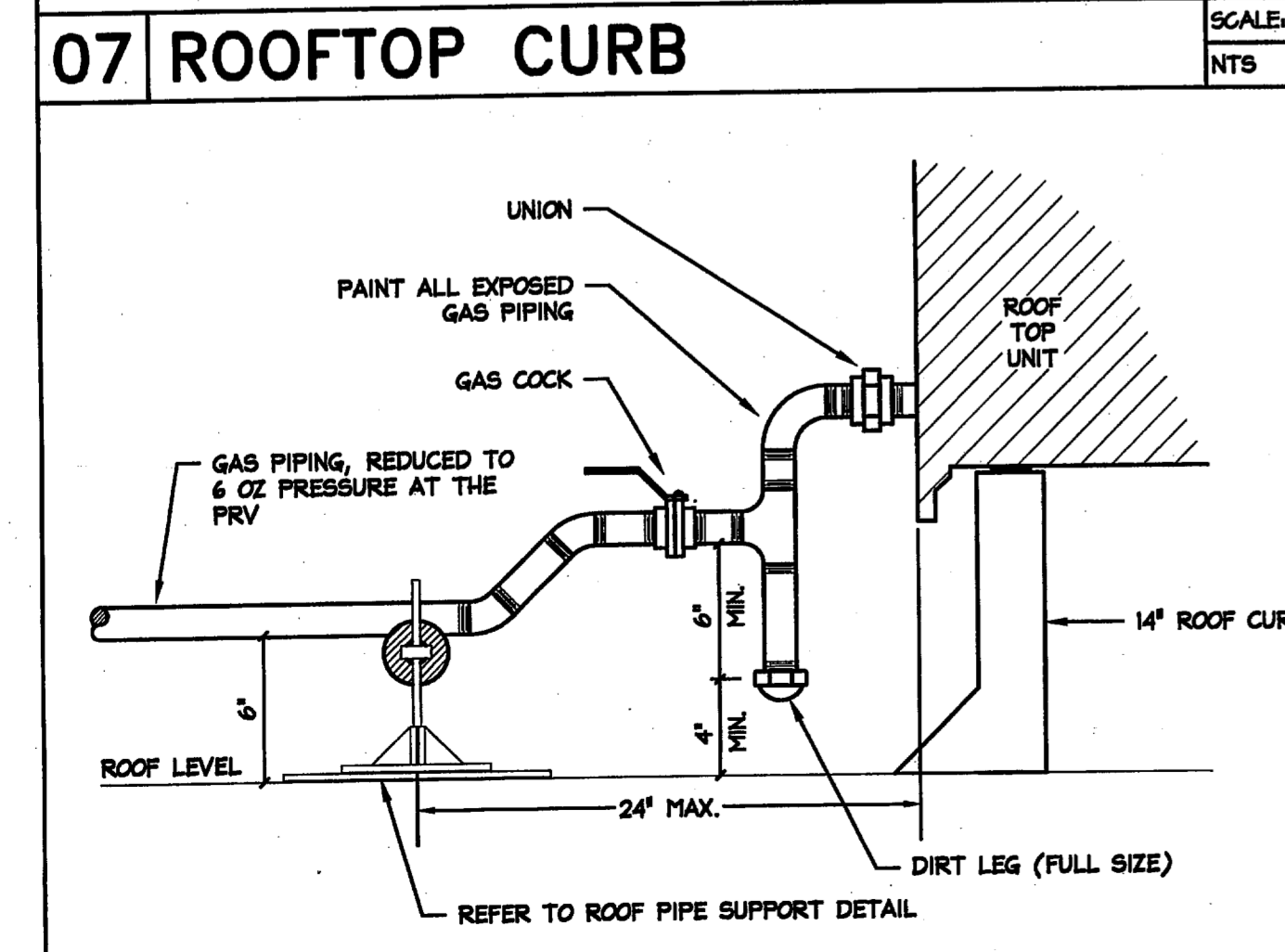
10 EQUIP. NAT. GAS CONN. DETAIL SCALE: NTS
