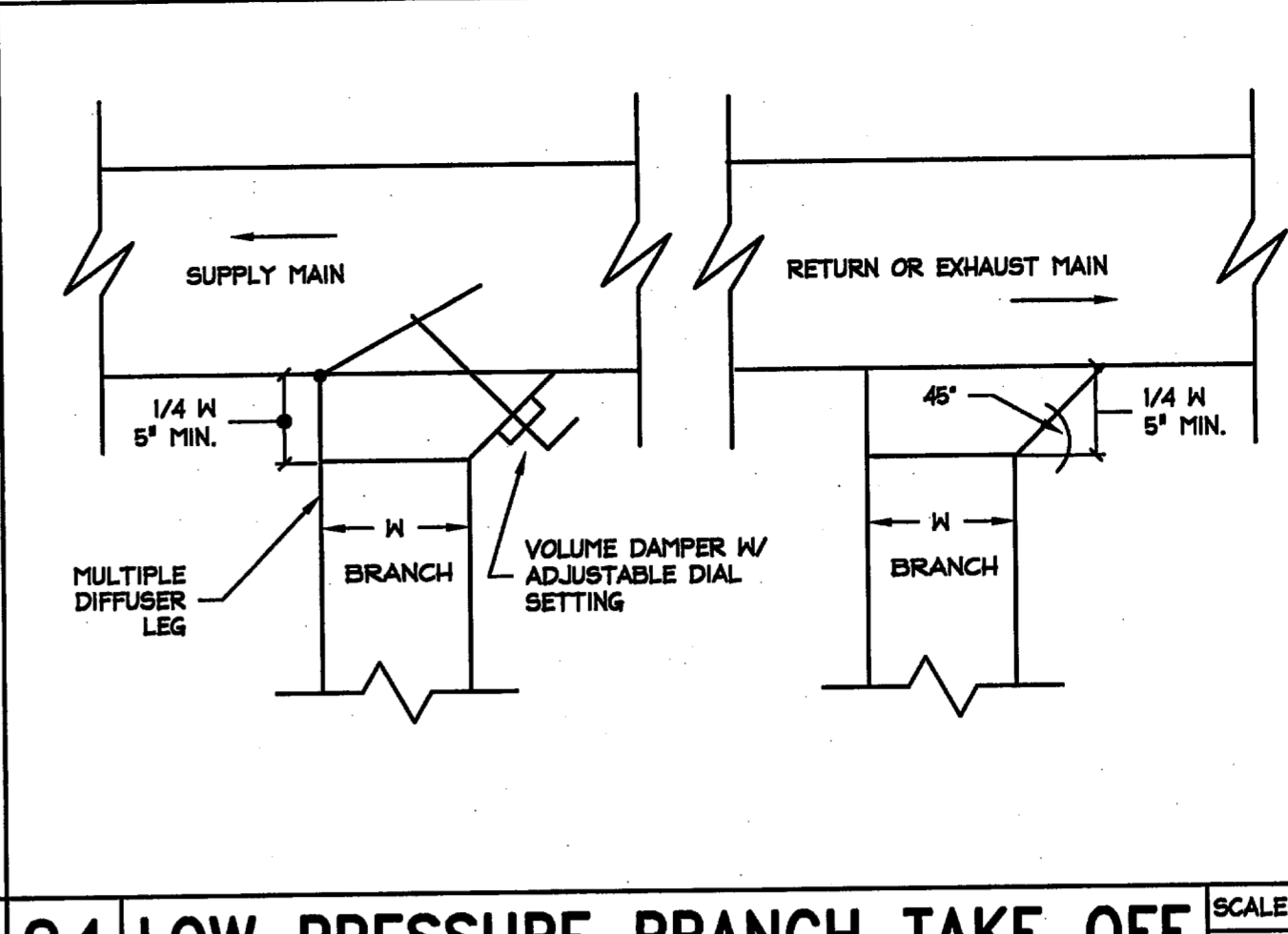
04 LOW PRESSURE BRANCH TAKE OFF SCALE: NTS
