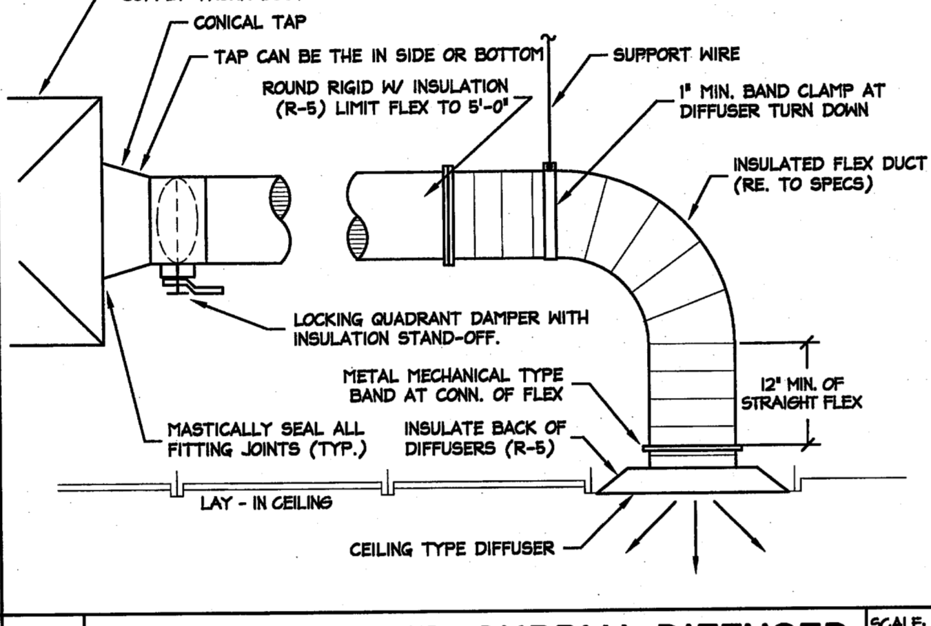
06 TYPICAL CEILING SUPPLY DIFFUSER SCALE: NTS
