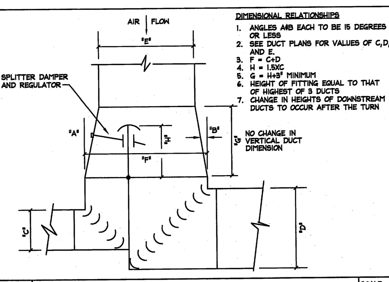
02 MAJOR RECTANGULAR DUCT TEE SCALE: NTS
