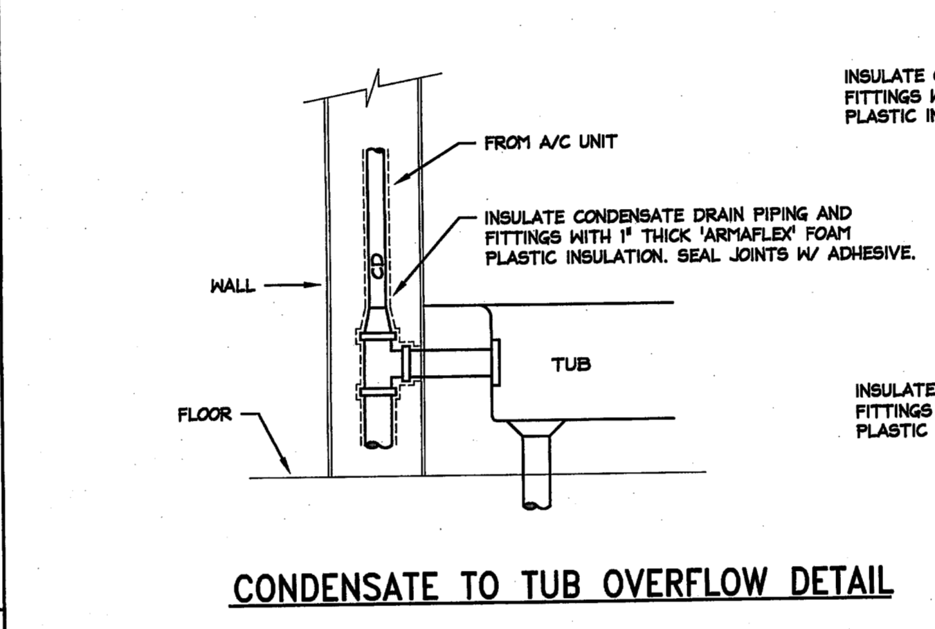
CONDENSATE TO TUB OVERFLOW DETAIL
