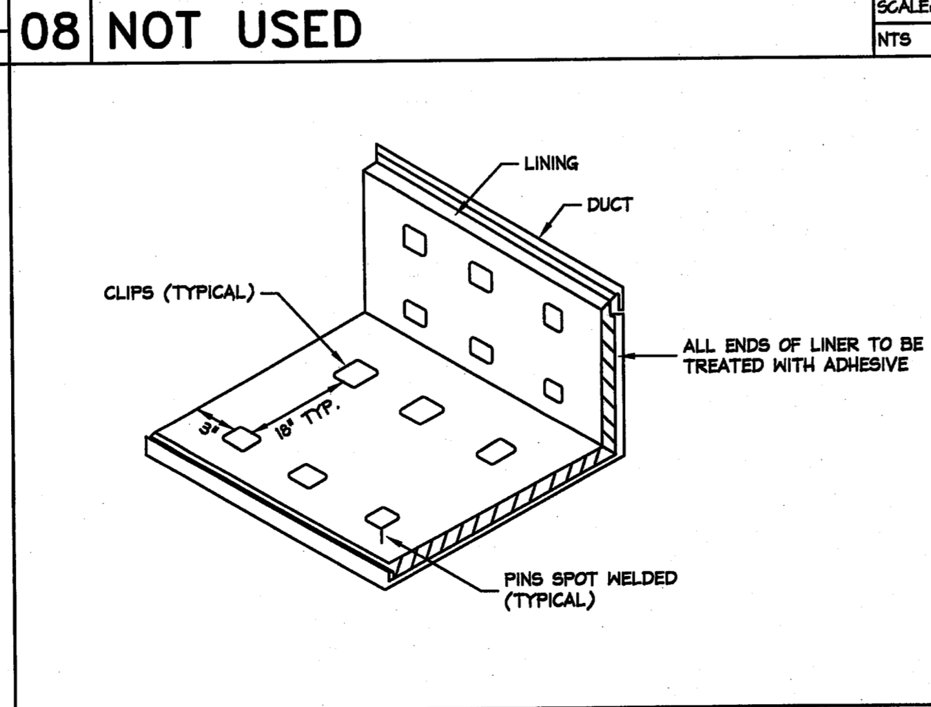
11 ACOUSTICAL DUCT LINING SCALE: NTS
