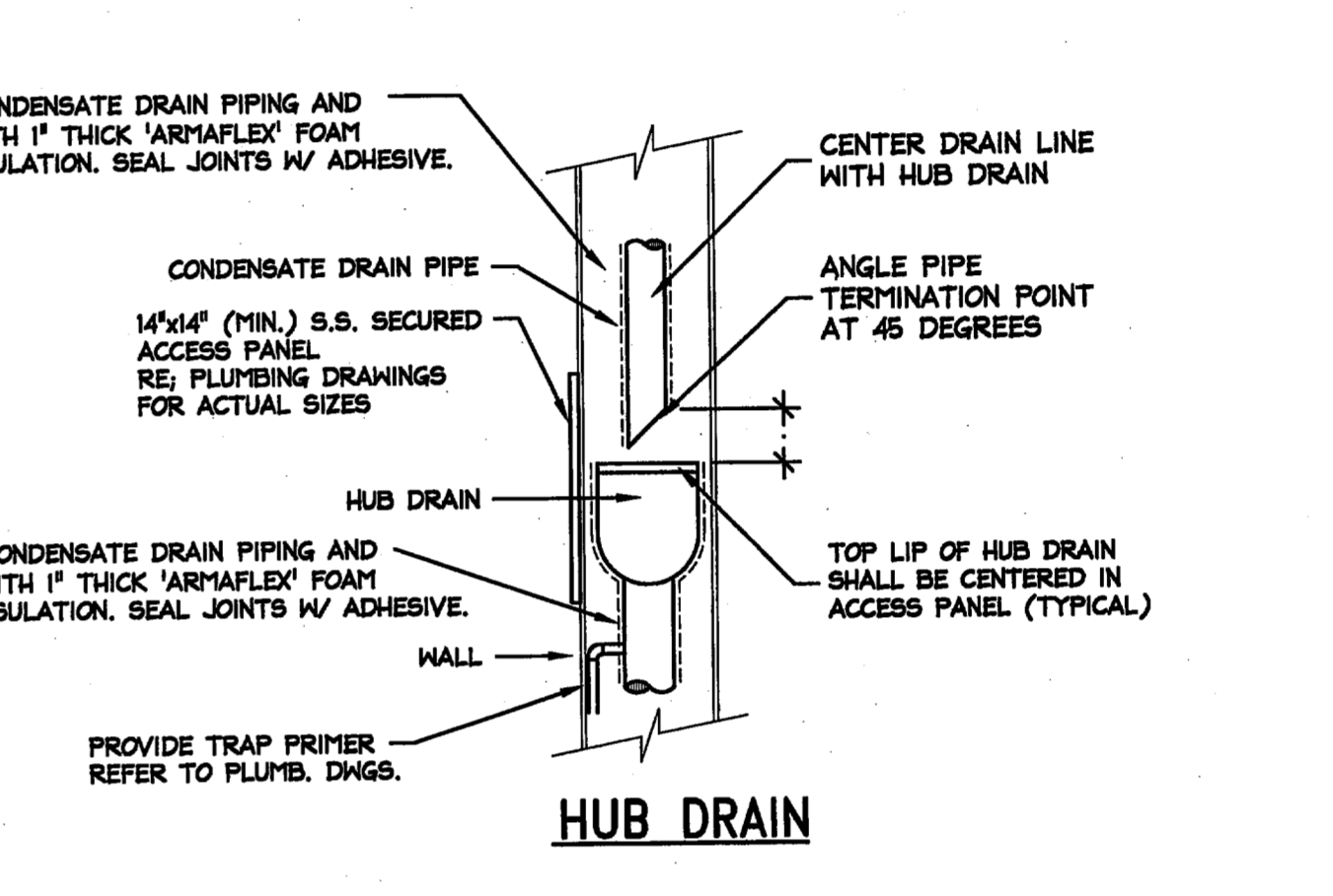
HUB DRAIN
