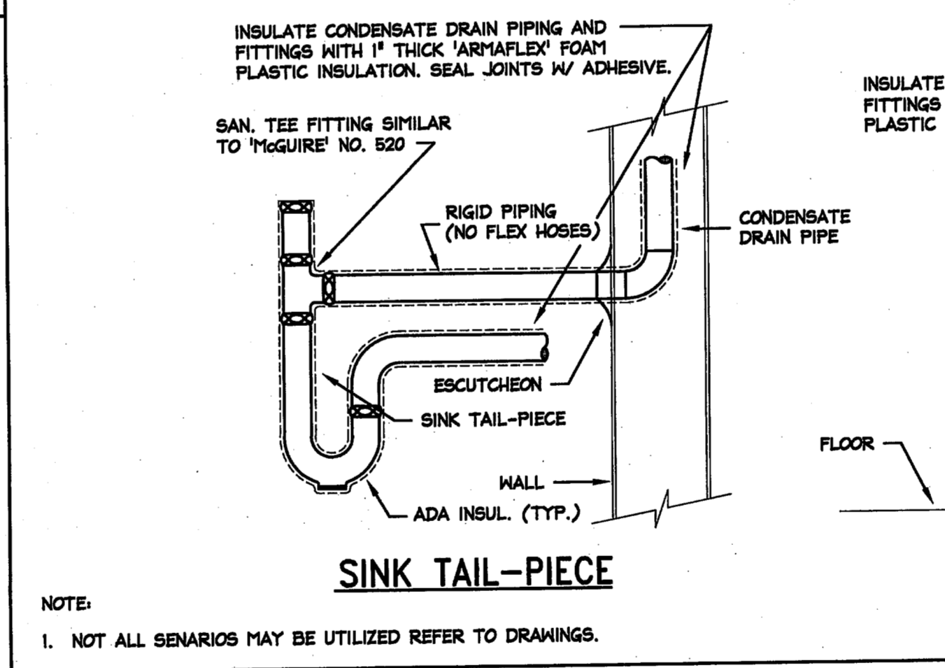
09 CONDENSATE PIPE TERMINATIONS DETAIL SCALE: NTS
