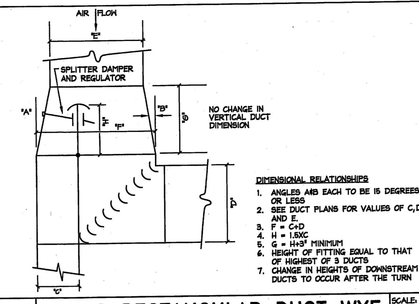
03 MAJOR RECTANGULAR DUCT WYE SCALE: NTS
