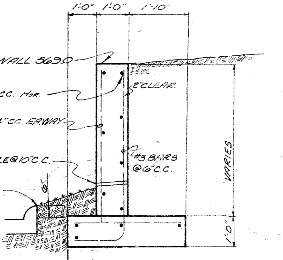
RETAINING WALL SECTION SCALE 1/2" = 1'-0"
