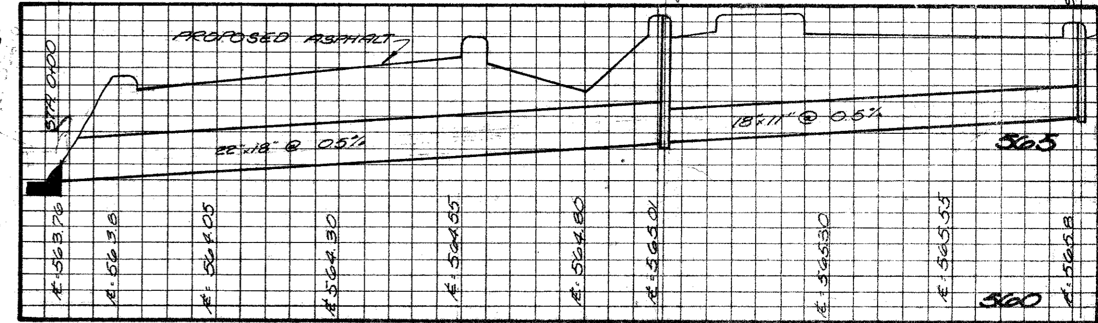
PROFILE STORM SEWER
