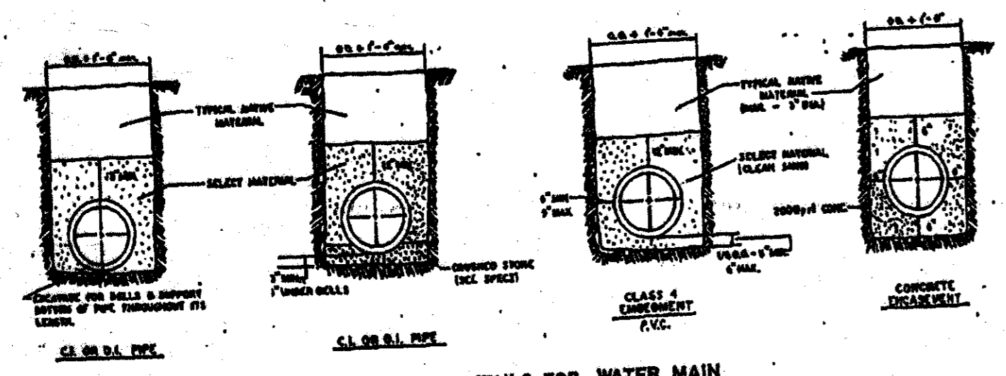
EMBEDMENT DETAILS FOR WATER MAIN
