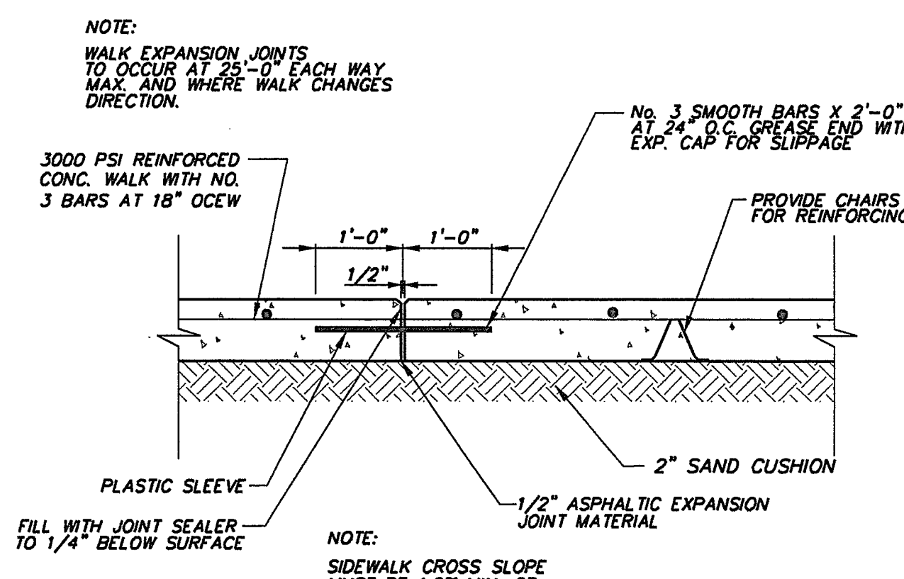
SIDEWALK EXPANSION JOINT NOT TO SCALE
