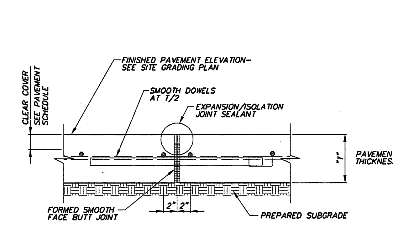
TRANSVERSE EXPANSION JOINT NOT TO SCALE
