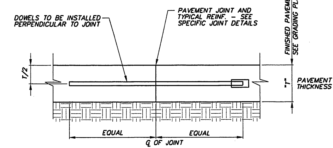
SMOOTH DOWEL NOT TO SCALE
