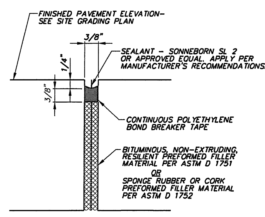
EXPANSION / ISOLATION JOINT SEALANT NOT TO SCALE
