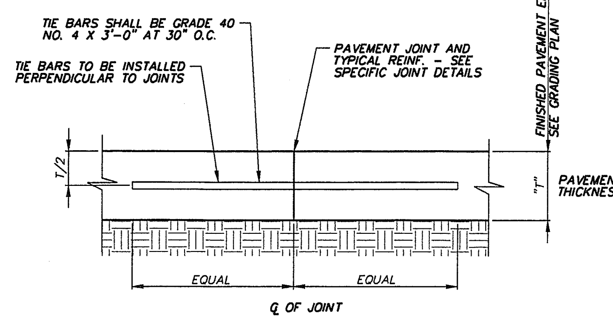
TIE BAR NOT TO SCALE
