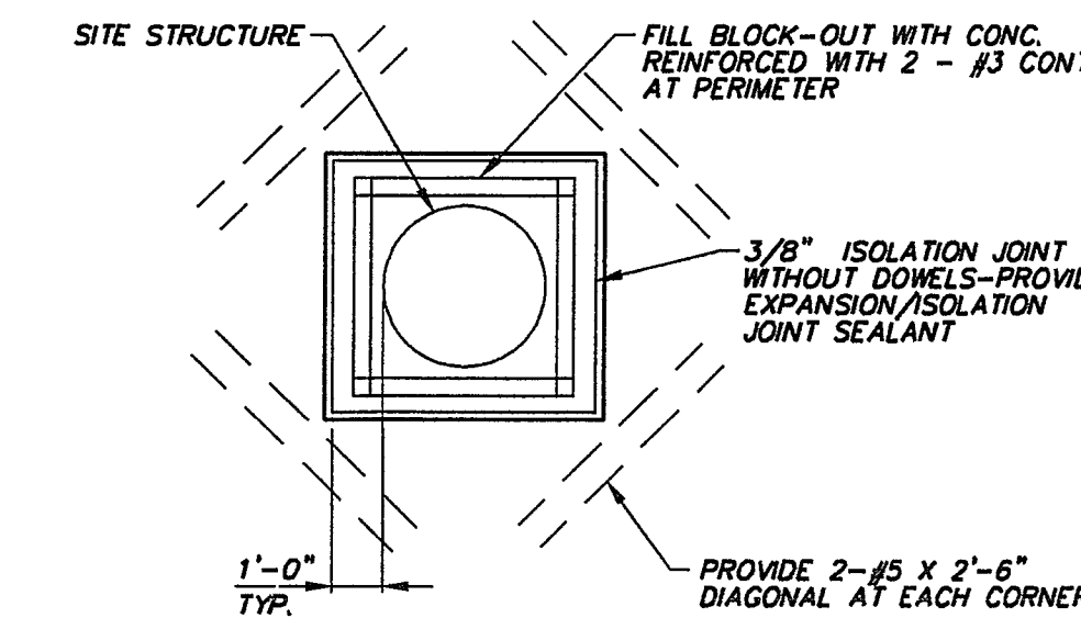
JOINT TREATMENT AT SITE STRUCTURES NOT TO SCALE
