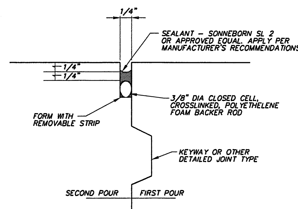
CONSTRUCTION JOINT SEALANT NOT TO SCALE
