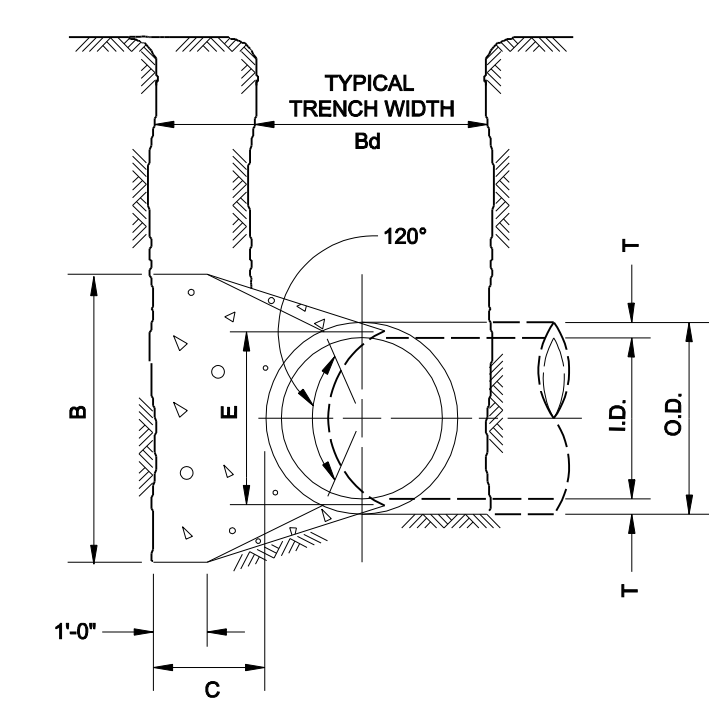
SECTION X-X
