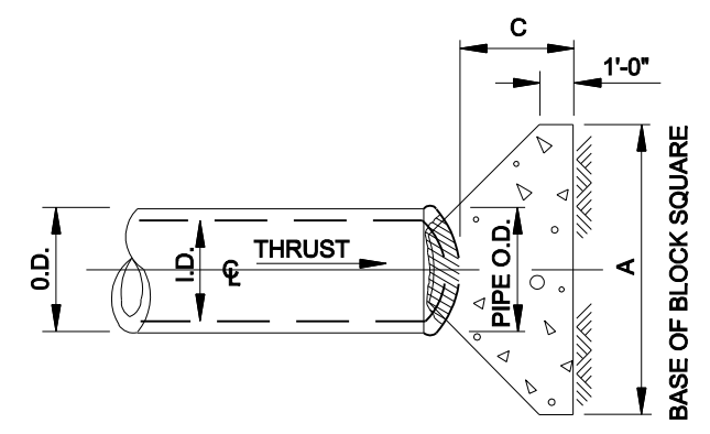
PLAN OF PLUG THRUST BLOCK
