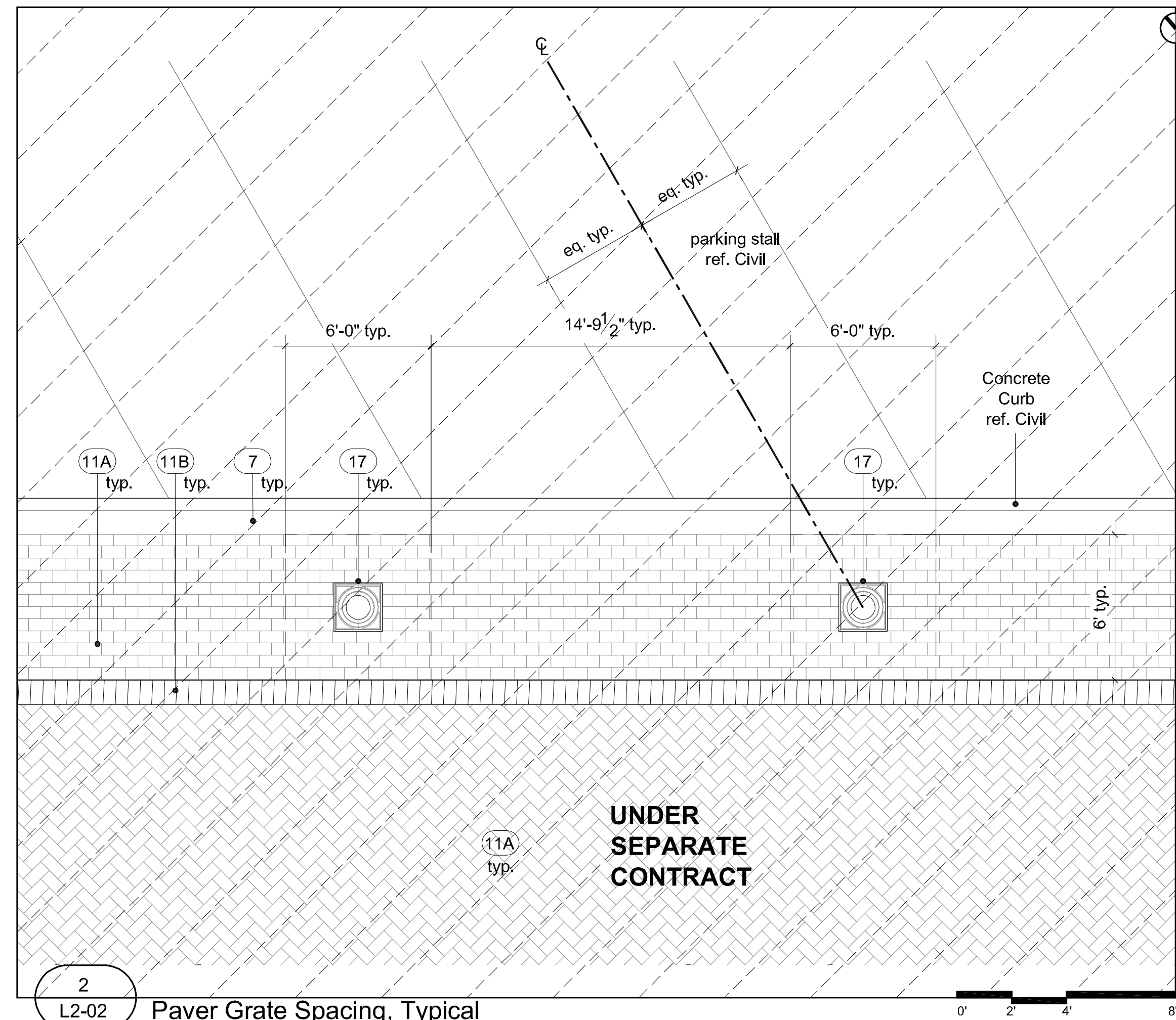
L2-02 Paver Grate Spacing, Typical
