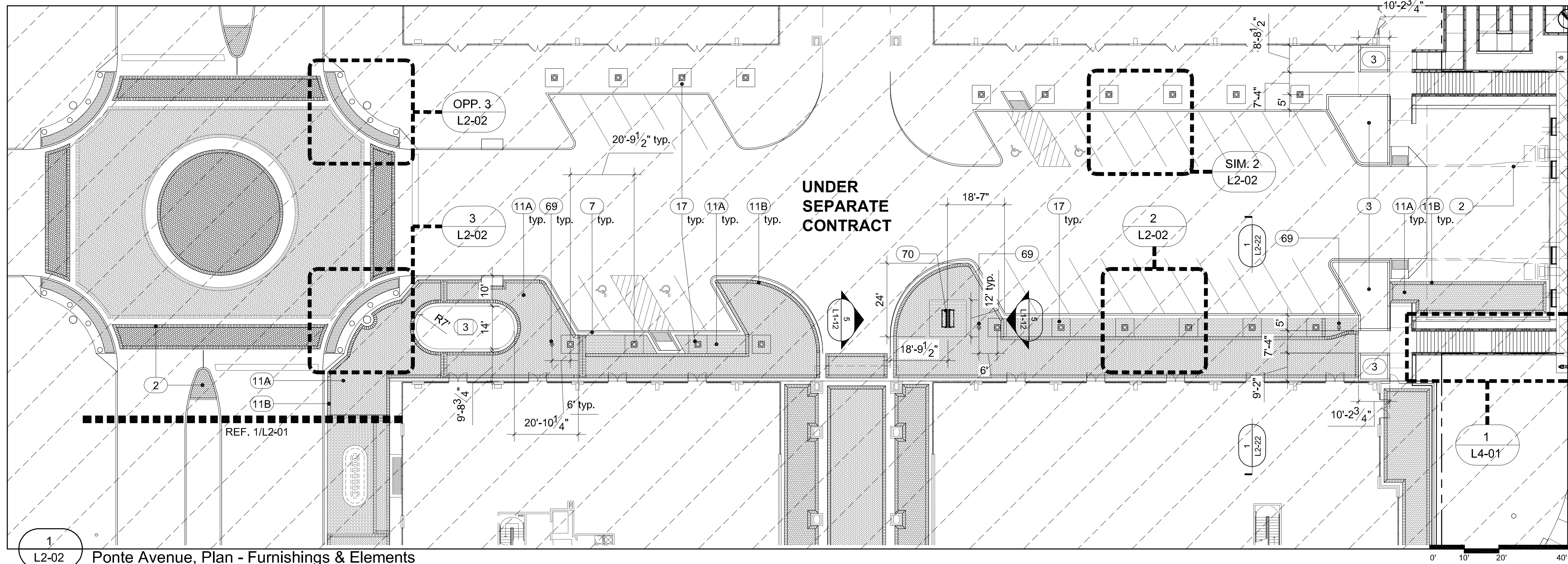
L2-02 Ponte Avenue, Plan - Furnishings & Elements
