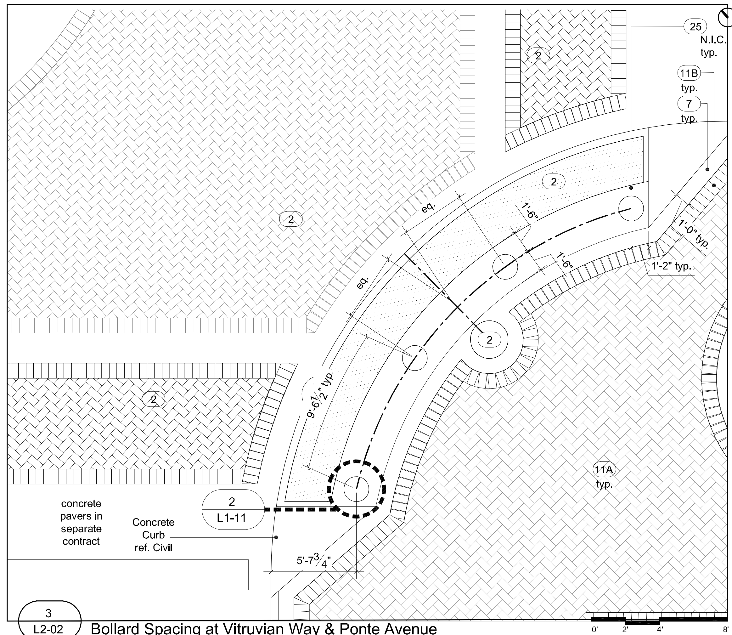
L2-02 Bollard Spacing at Vitruvian Way & Ponte Avenue
