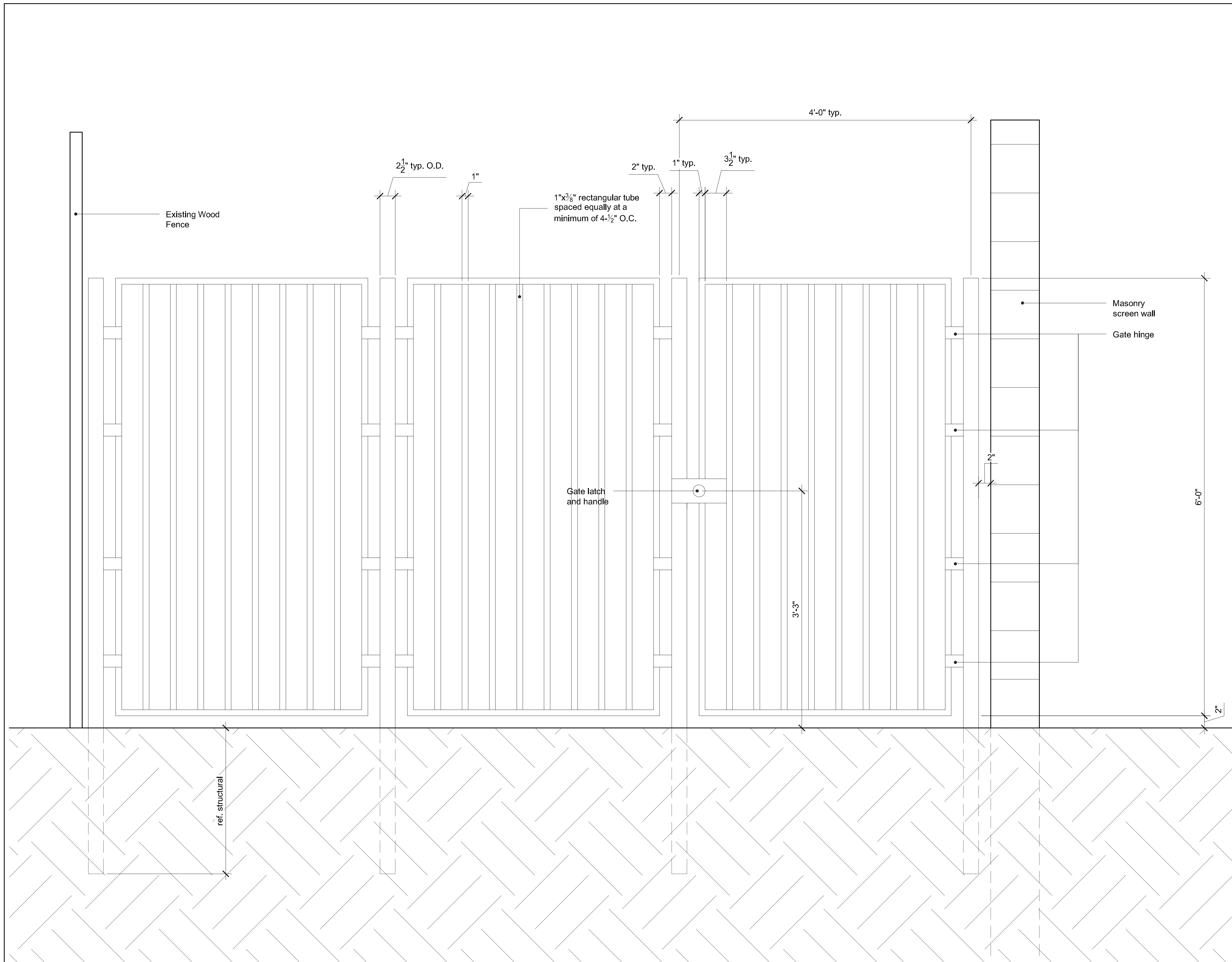
1 L3-04 Gate Elevation
