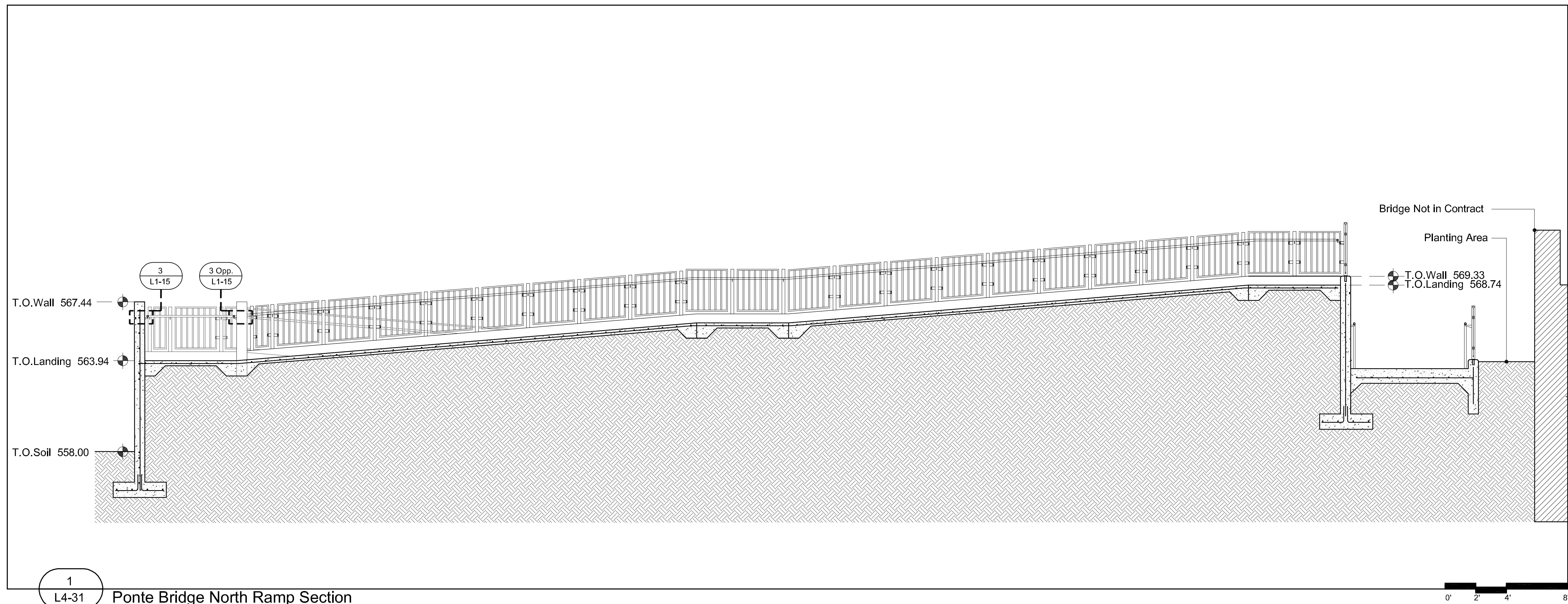
2 L4-31 Ponte Bridge North Ramp Section
