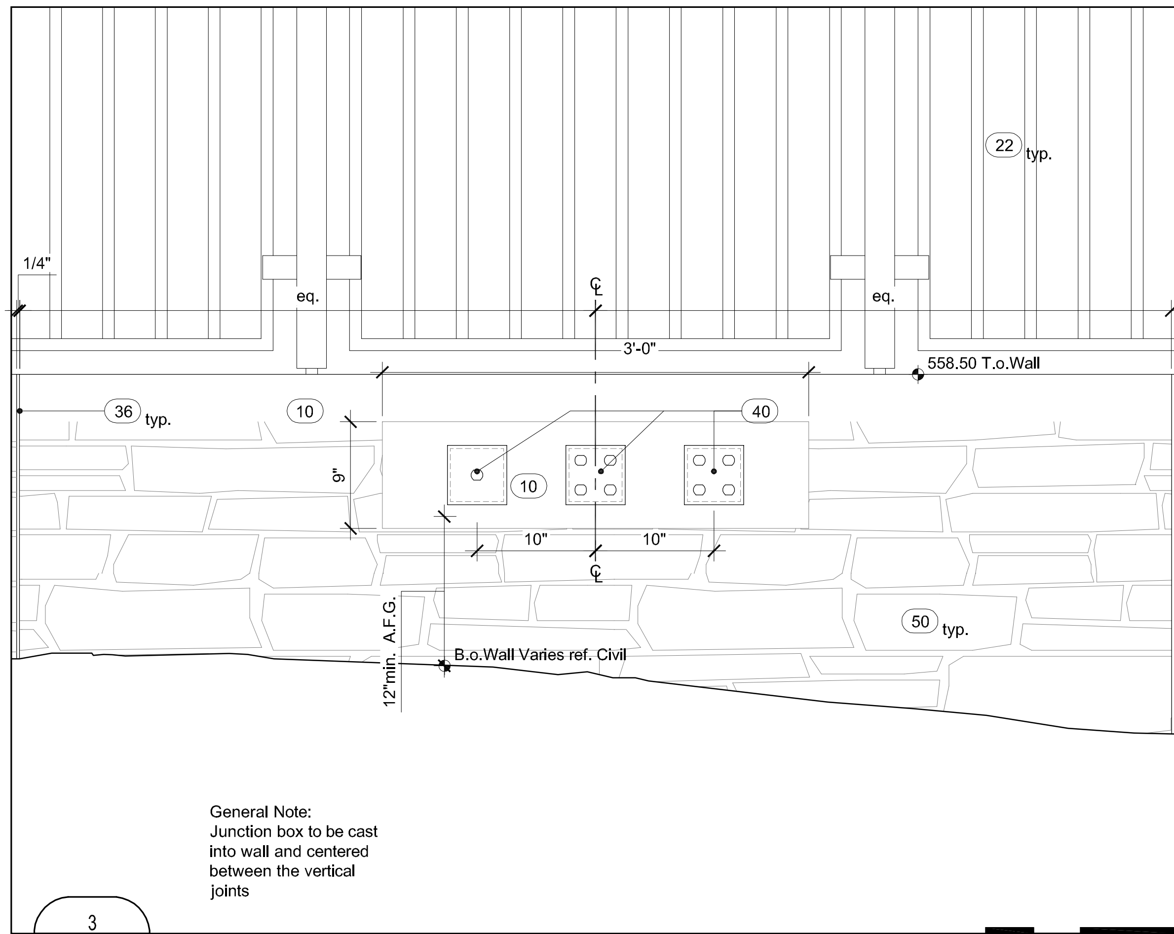
3 L5-04 Enlarged Wall Electrical Outlets Detail
