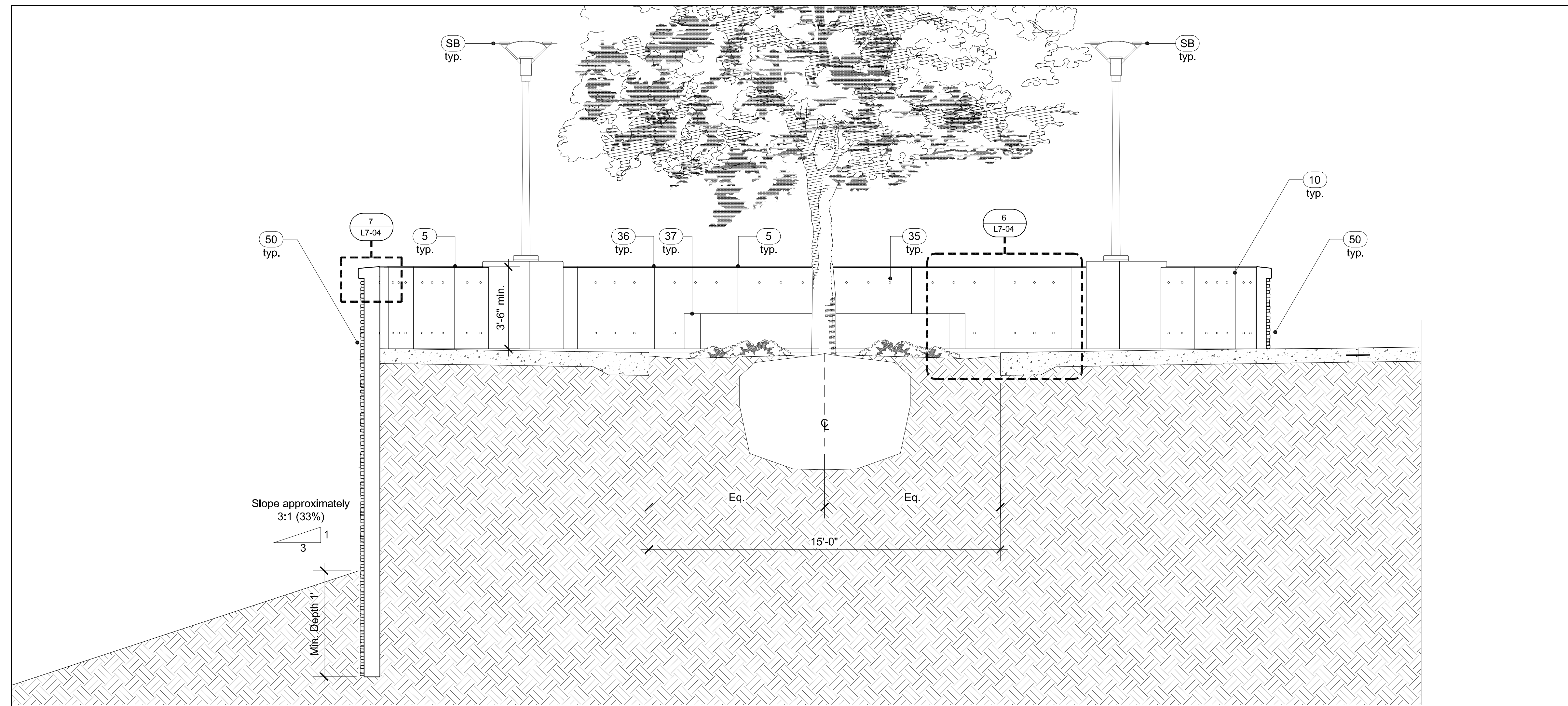
1 L7-03 Belvedere - Section
