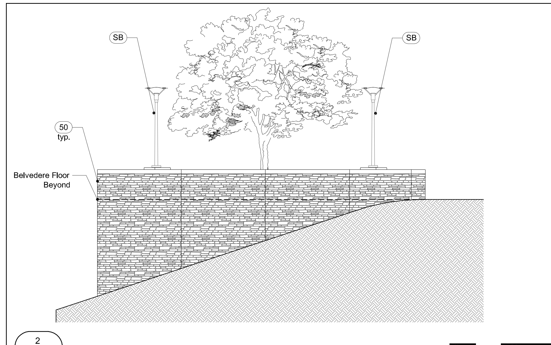
2 L7-03 Belvedere - Elevation
