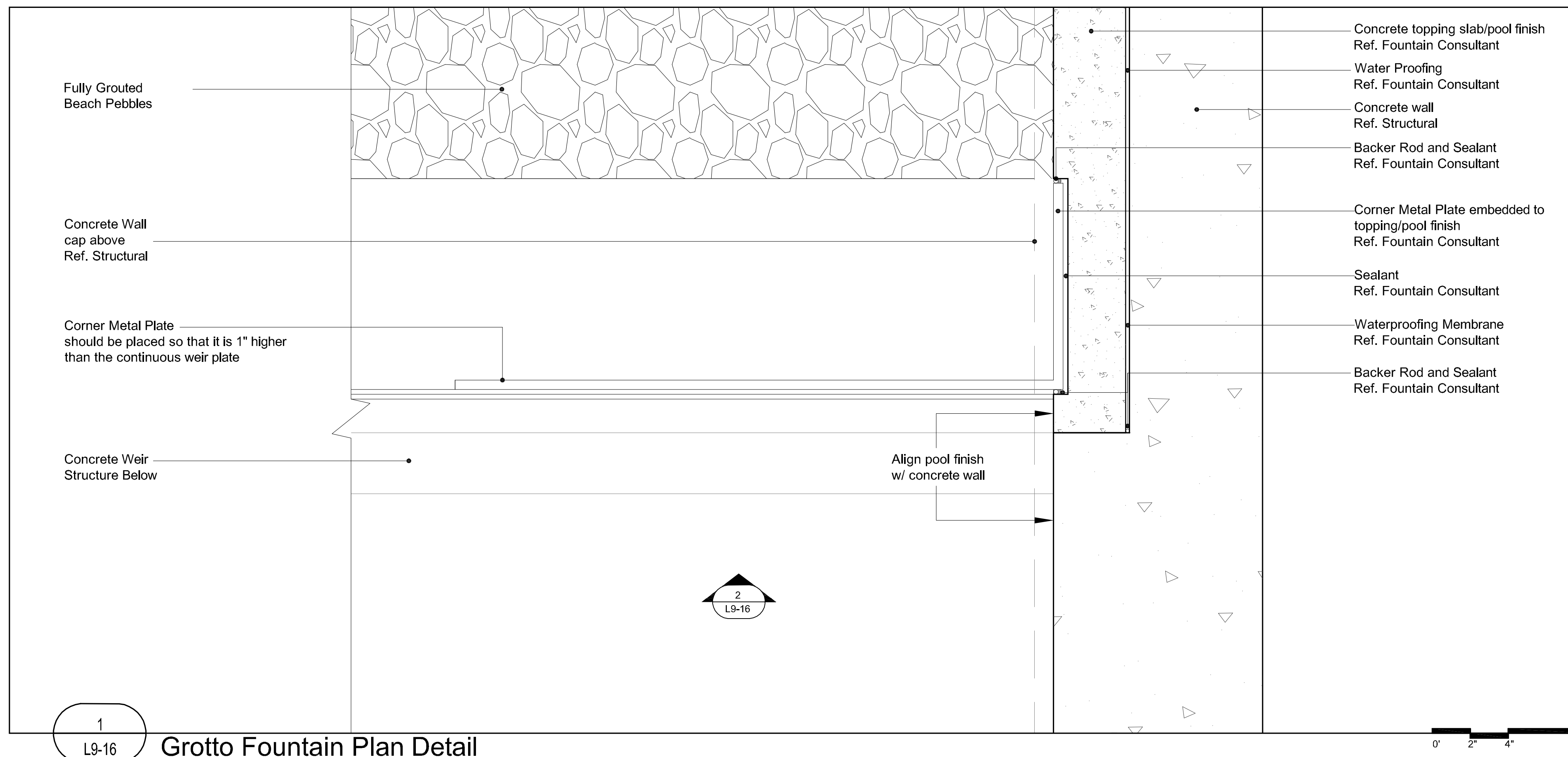
Grotto Fountain Detail - Elevation
