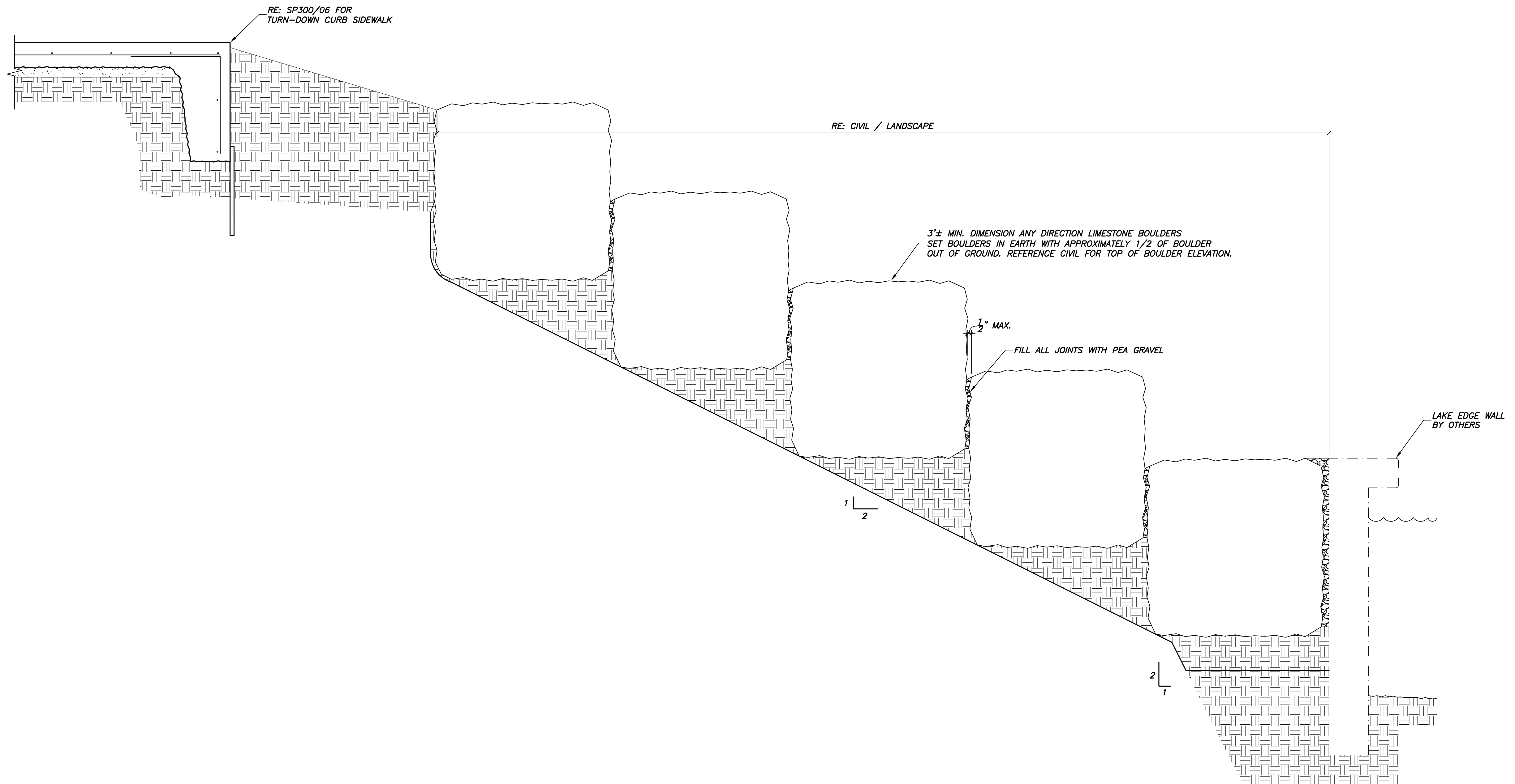
01 SECTION 1"=1'-0"
