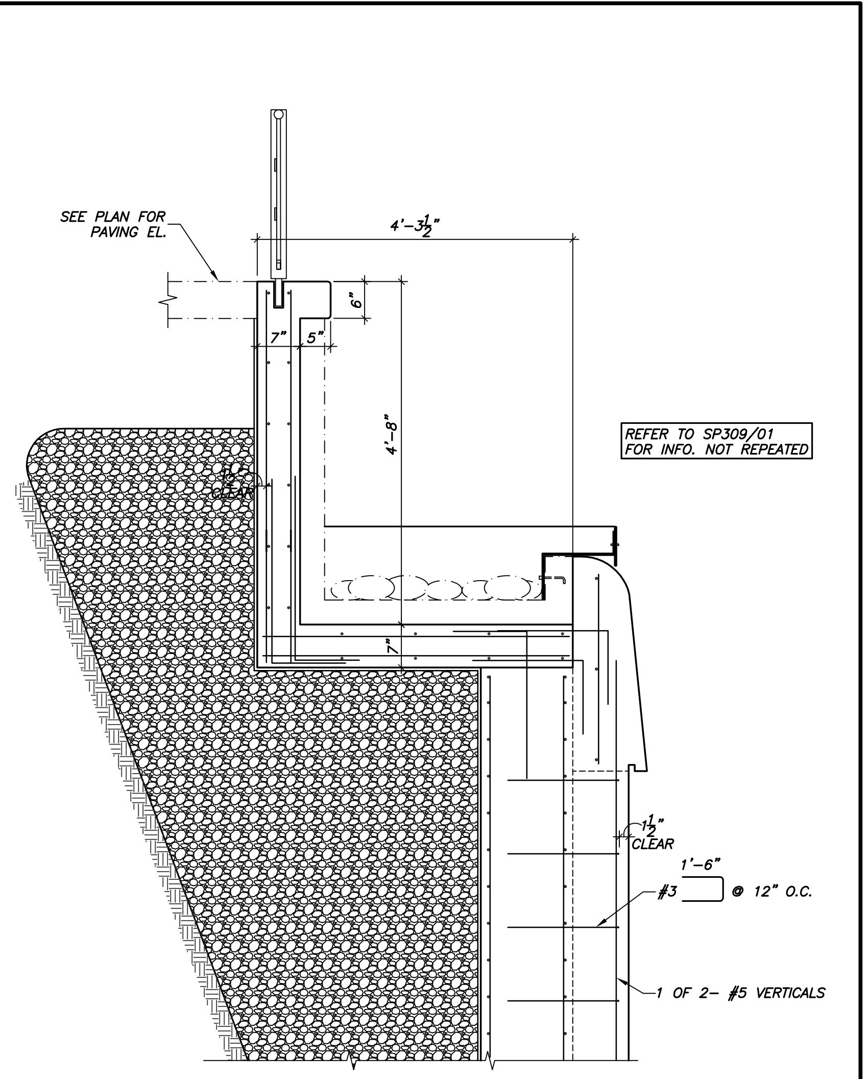
03 SECTION 3/4'-1'-0"
