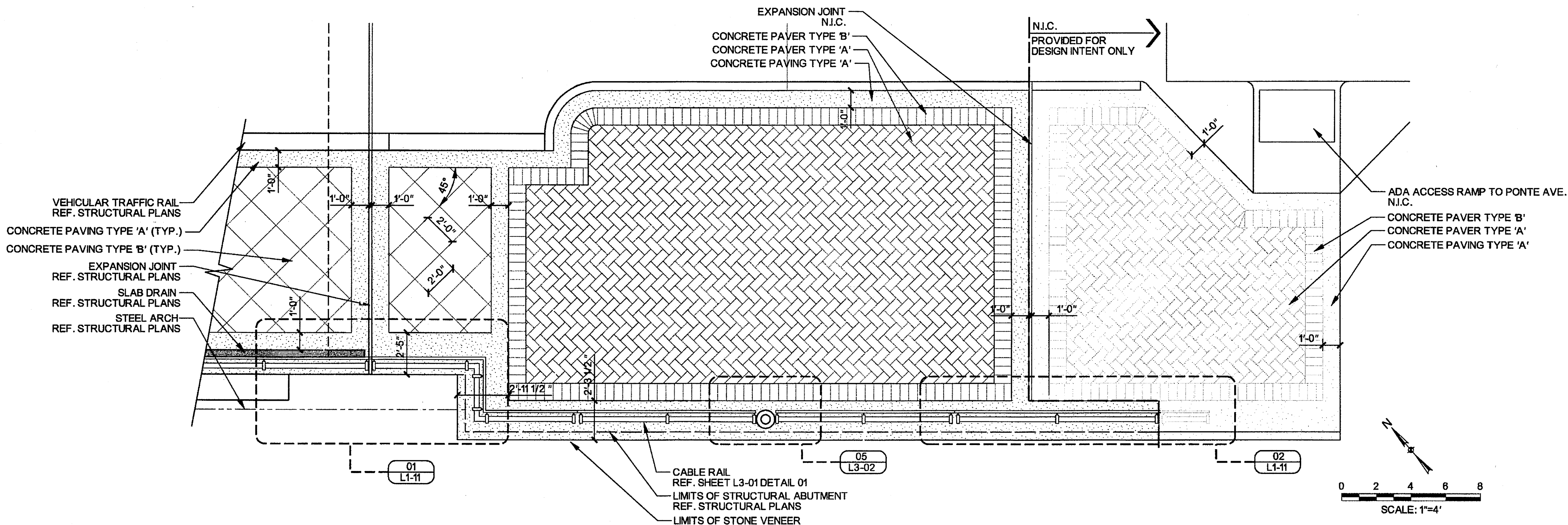
02 PAVING LAYOUT-SOUTH APPROACH (TYP.) PLAN
