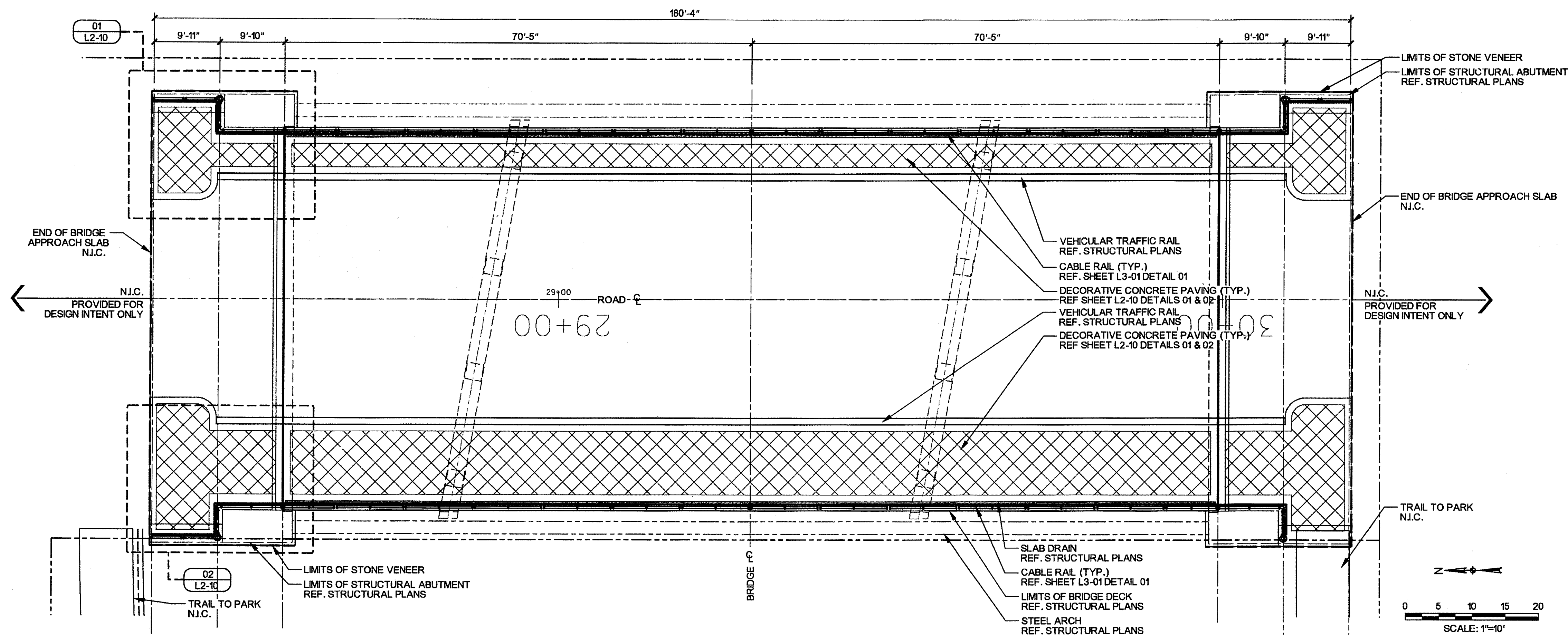
01 CABLE RAIL AND PAVING LAYOUT SCALE: 10"=1'-0" PLAN
