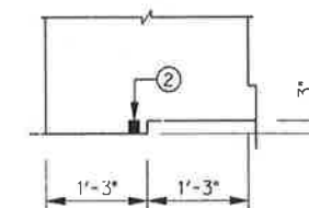
BOTTOM CONST JT DETAIL SCALE: NTS
