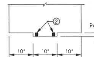
TOP CONST JT DETAIL SCALE: NTS
