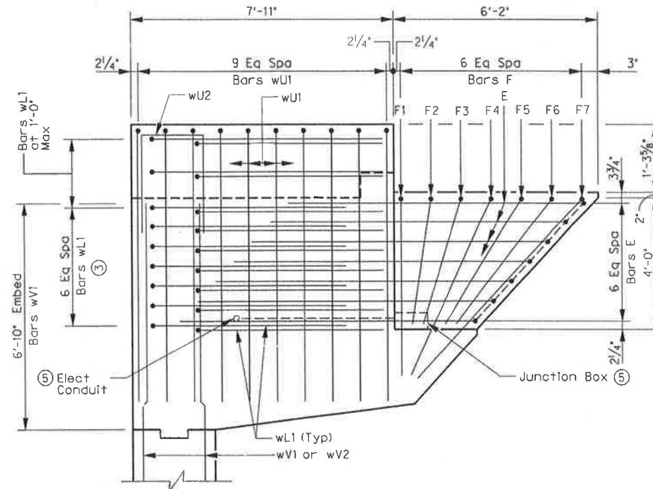
MASK WALL DETAIL SCALE: 1/2" = 1'-0"
