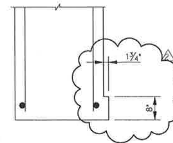
STONE LEDGE DETAIL OFF OF CAP SCALE: NTS
