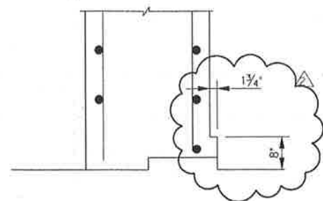
STONE LEDGE DETAIL AT CAP SCALE: NTS
