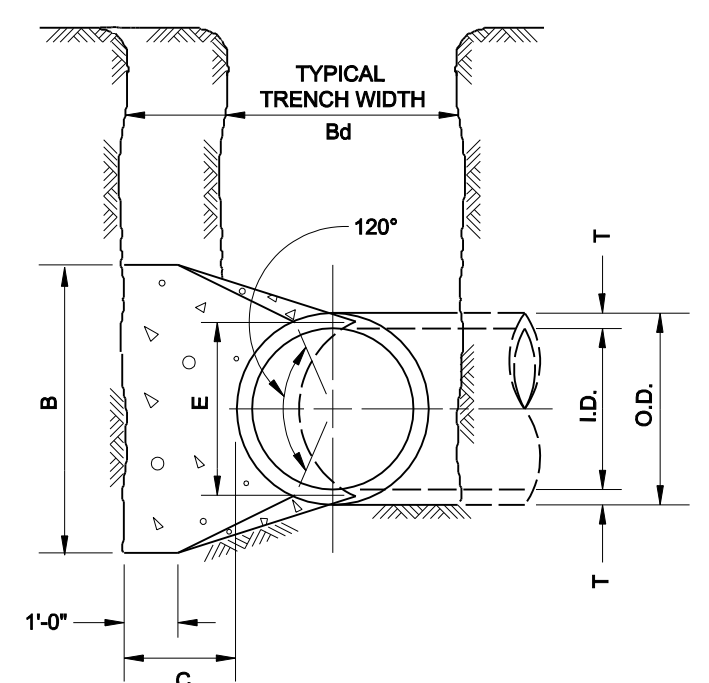
SECTION X-X
