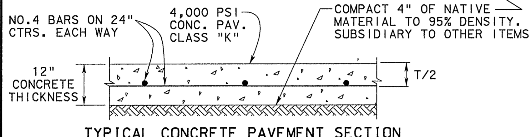
TYPICAL CONCRETE PAVEMENT SECTION N.T.S.
