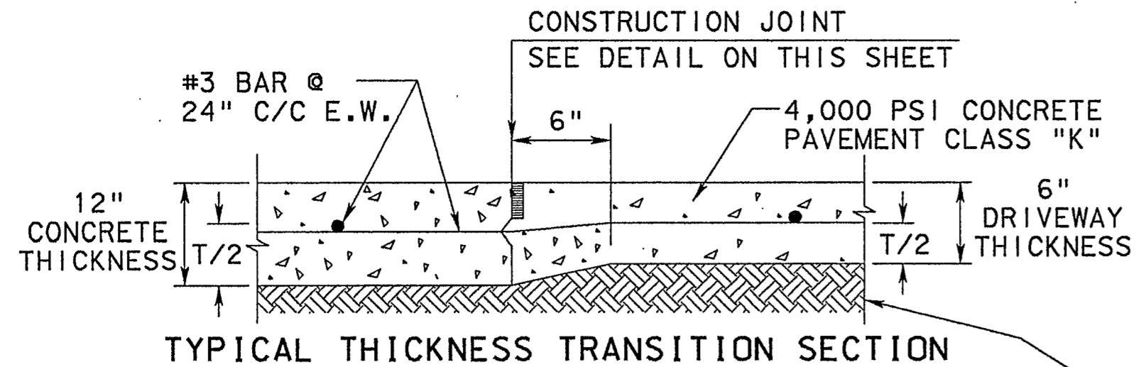
TYPICAL THICKNESS TRANSITION SECTION N.T.S.
