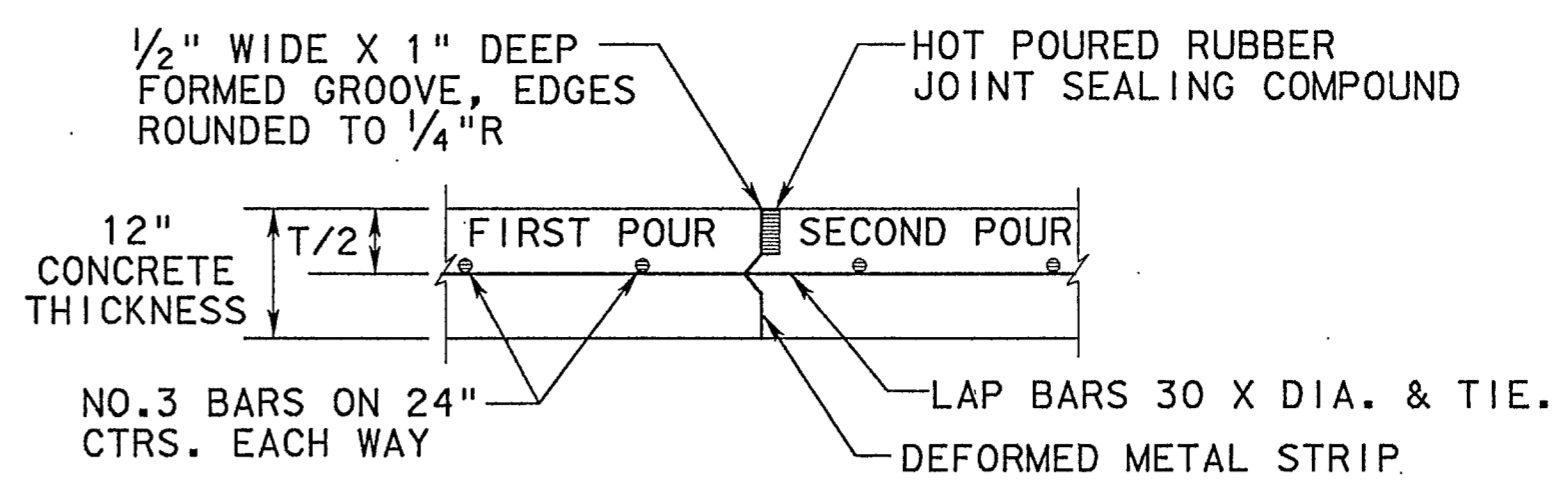
CONSTRUCTION JOINT DETAIL N.T.S.
