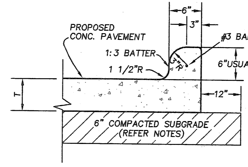
03 INTEGRAL 6" CURB SECTION NOT TO SCALE
