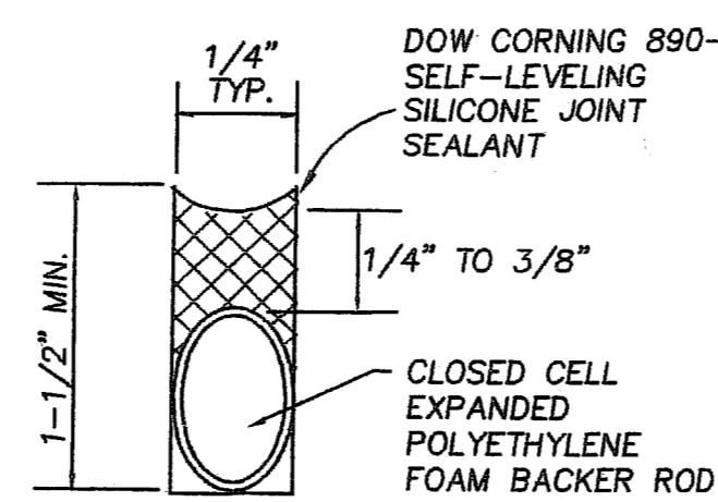
06 JOINT SEAL DETAIL NOT TO SCALE
