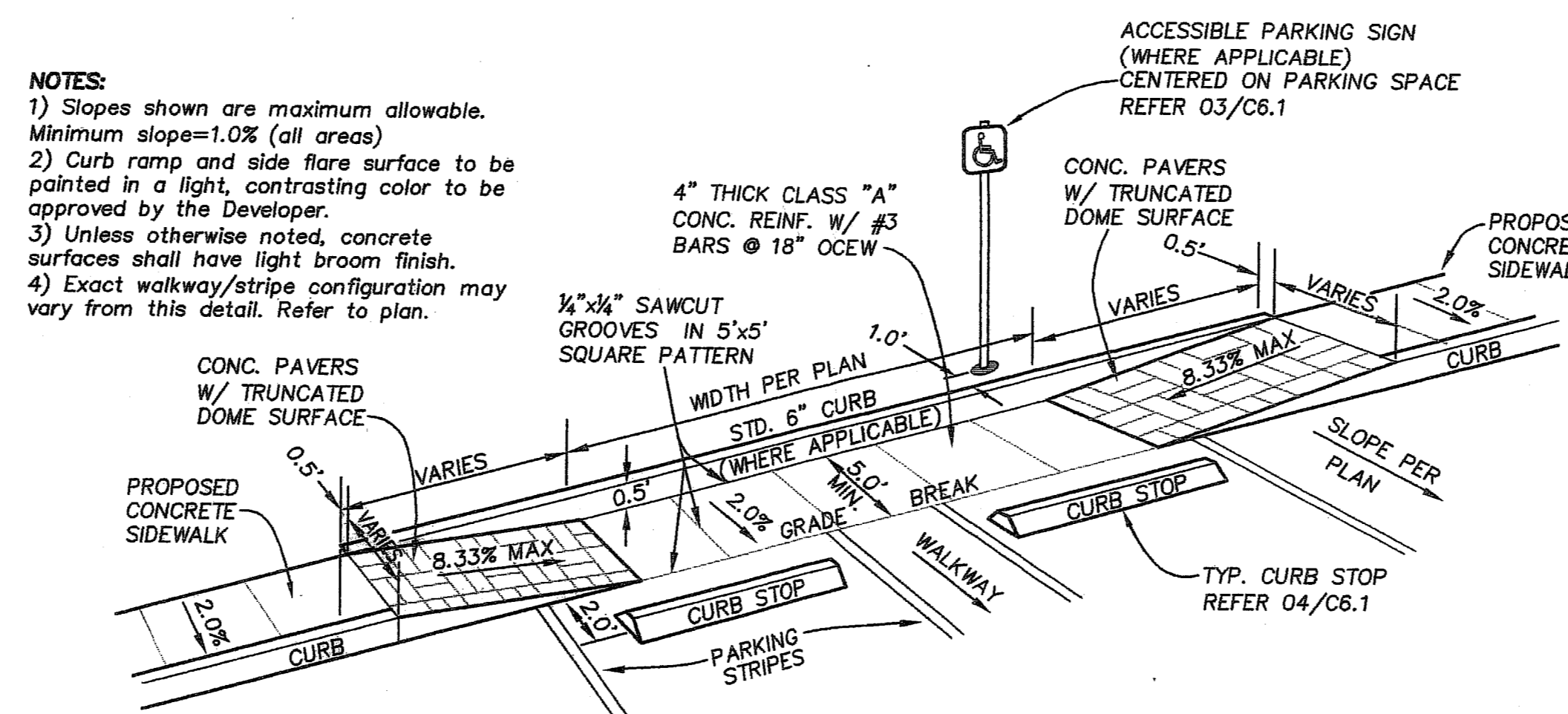
12 TYPE 2 CURB RAMP & PARKING DETAIL NOT TO SCALE
