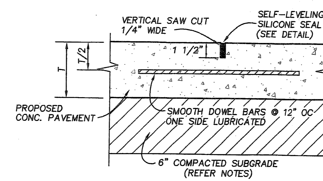
08 LONGITUDINAL OR TRANSVERSE DOWELED CONTRACTION JOINT NOT TO SCALE
