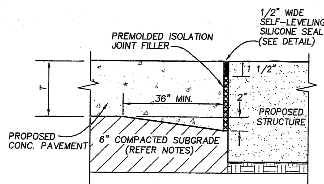
09 ISOLATION JOINT NOT TO SCALE
