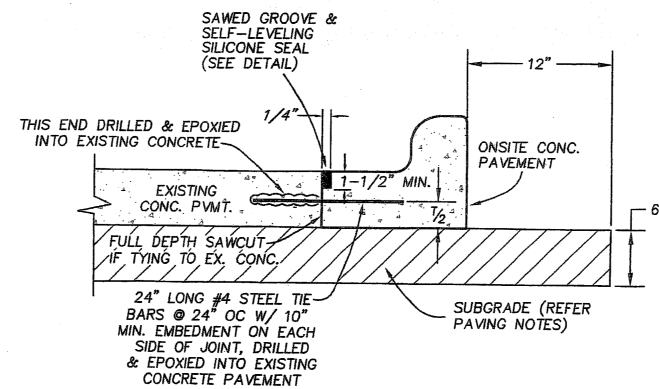
07 CONC. PVMT. CONNECTION @ CURB NOT TO SCALE
