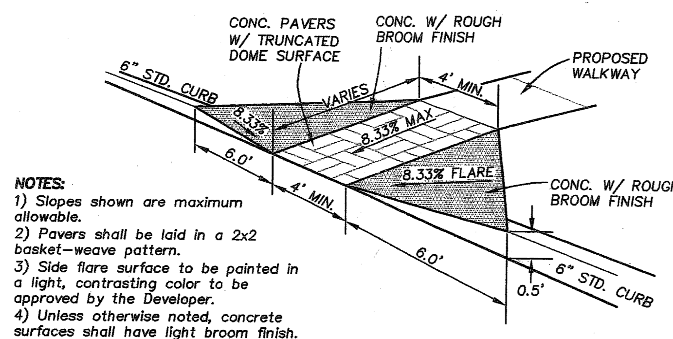
11 TYPE 1 CURB RAMP DETAIL NOT TO SCALE
