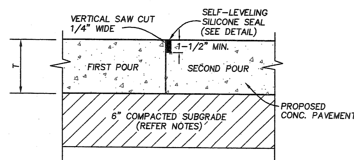
02 LONGITUDINAL OR TRANSVERSE CONSTRUCTION JOINT NOT TO SCALE
