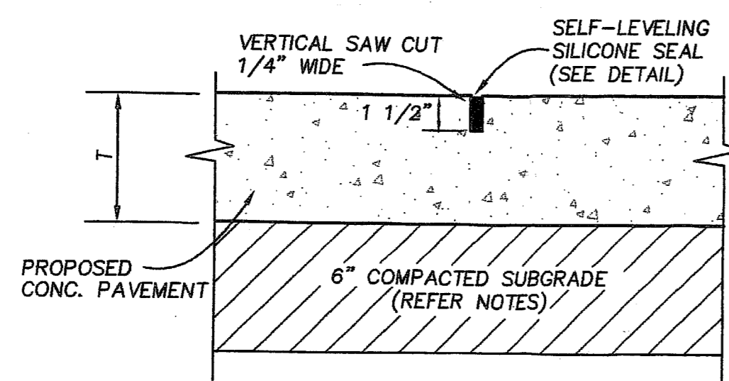
05 LONGITUDINAL OR TRANSVERSE CONTRACTION JOINT NOT TO SCALE
