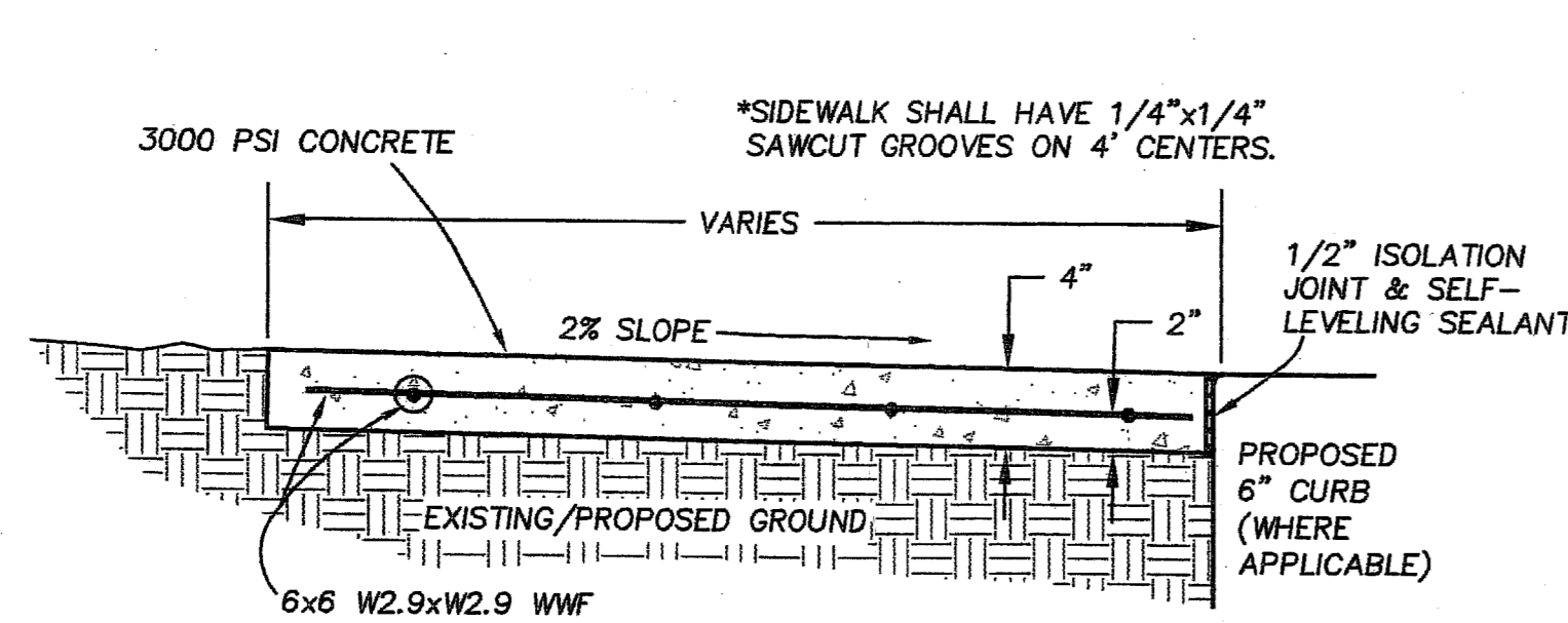
01 SIDEWALK DETAIL NOT TO SCALE
