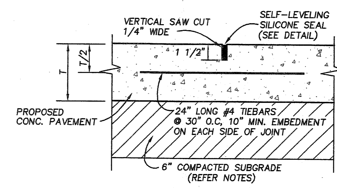
04 LONGITUDINAL OR TRANSVERSE TIED CONTRACTION JOINT NOT TO SCALE
