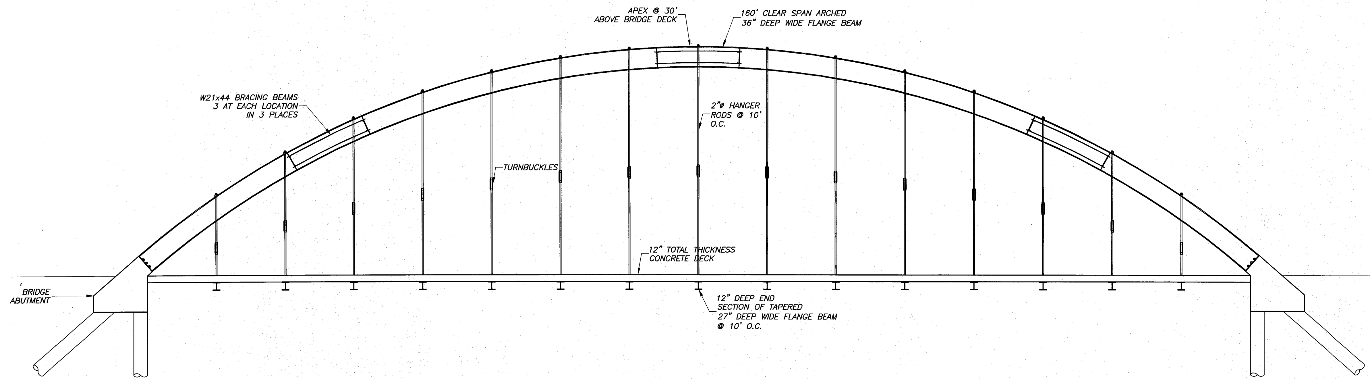
01 ELEVATION VIEW \frac{1}{8}'' = 1'-0''
