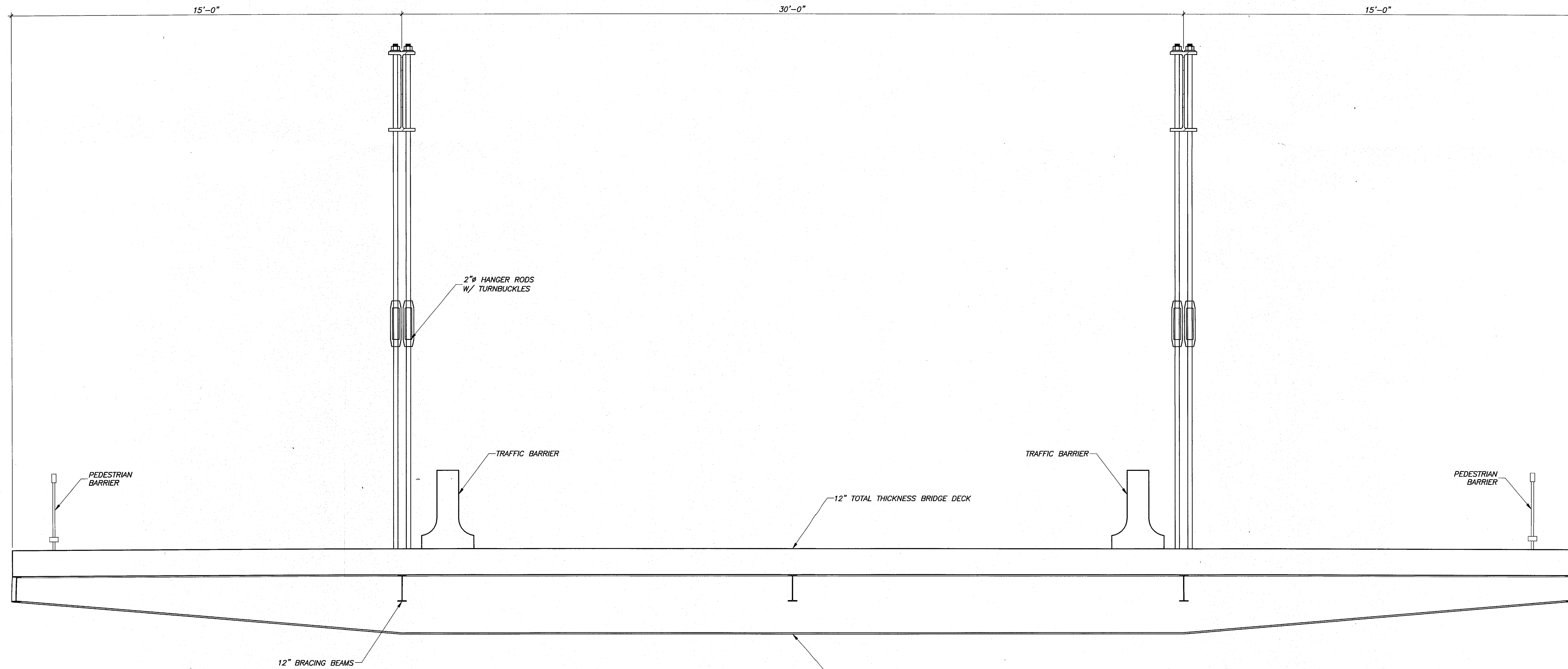
01 CROSS SECTION \frac{1}{2}'' = 1'-0''
