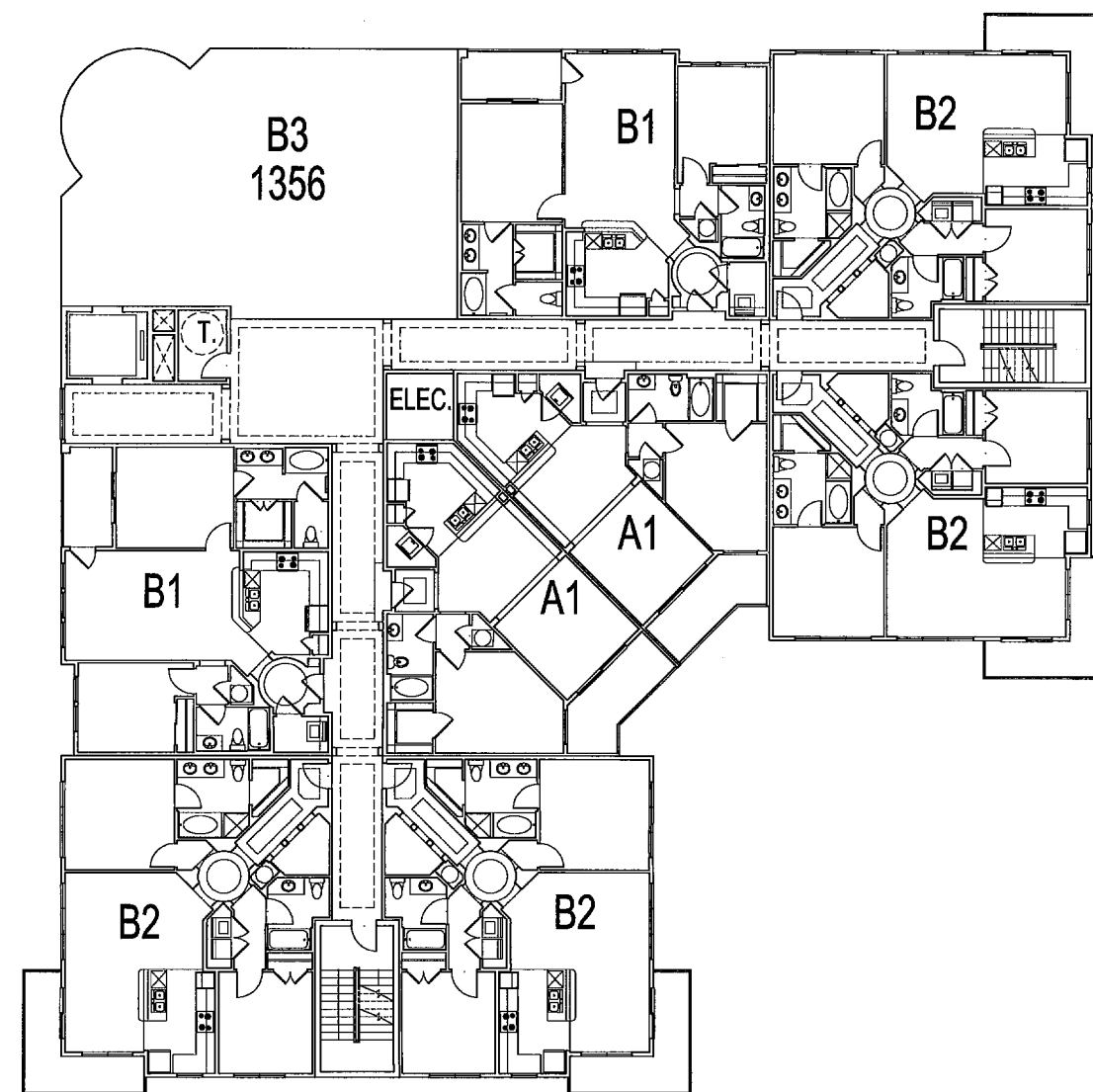
BUILDING-3 26 UNITS 3-STORY ON TOP OF PODIUM
