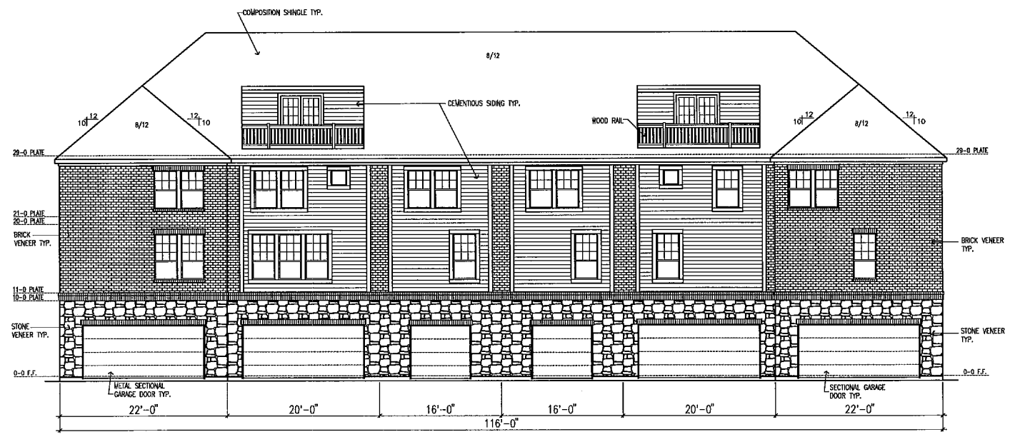
REAR ELEVATION
