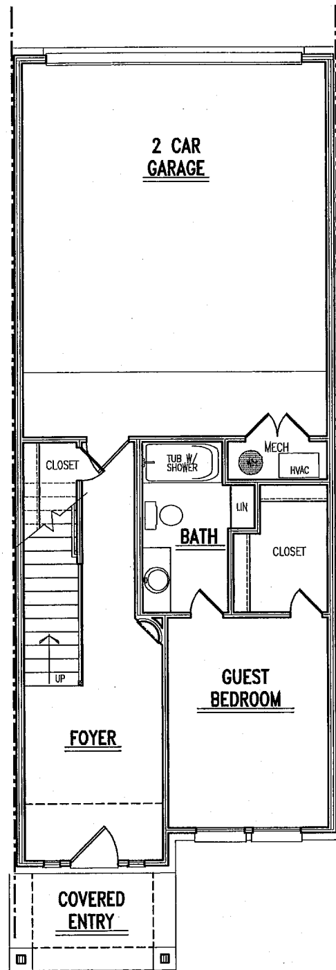
FIRST FLOOR PLAN- UNIT B
