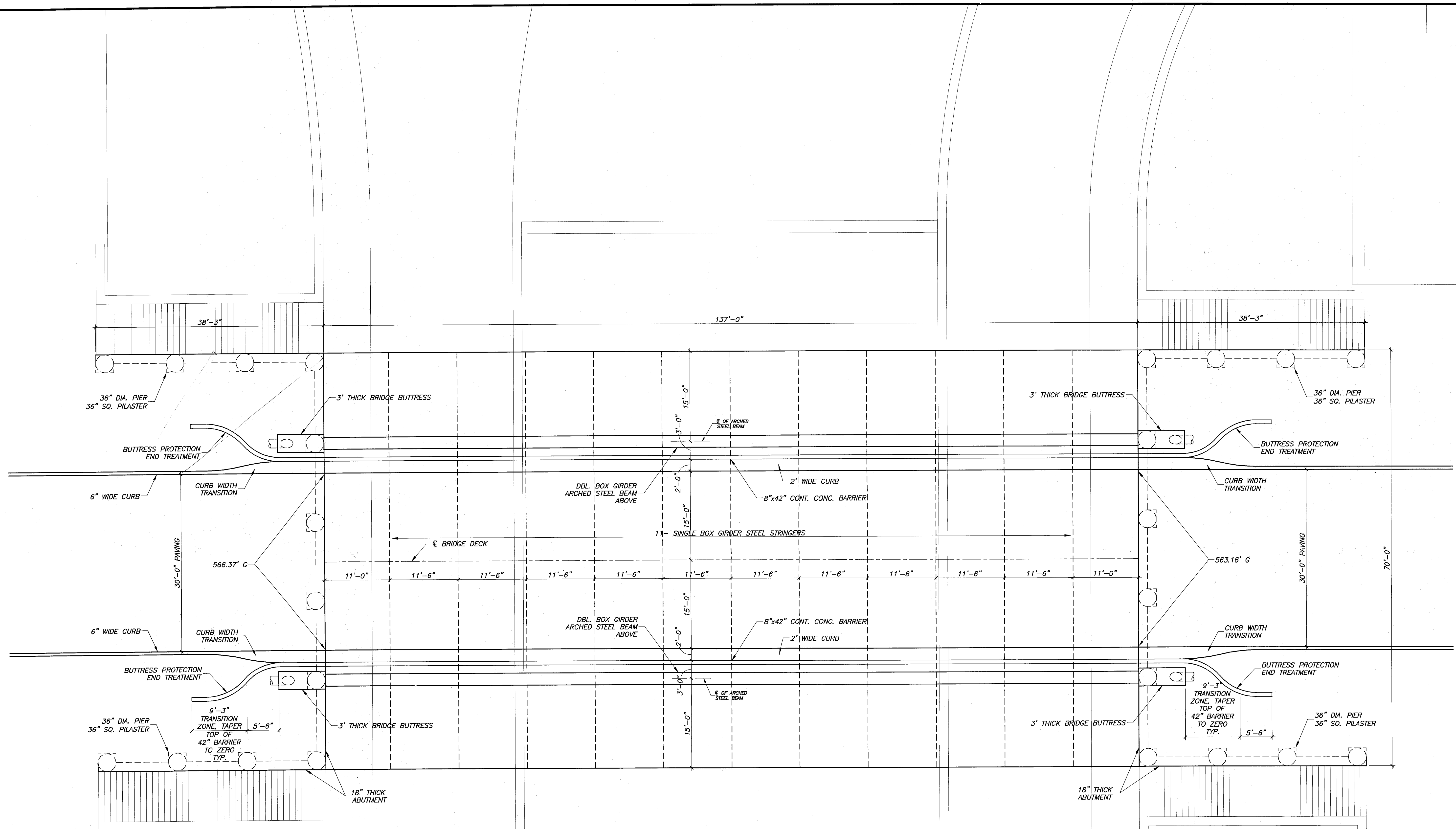
01 TRAFFIC BRIDGE PLAN 1/8" = 1'-0"
