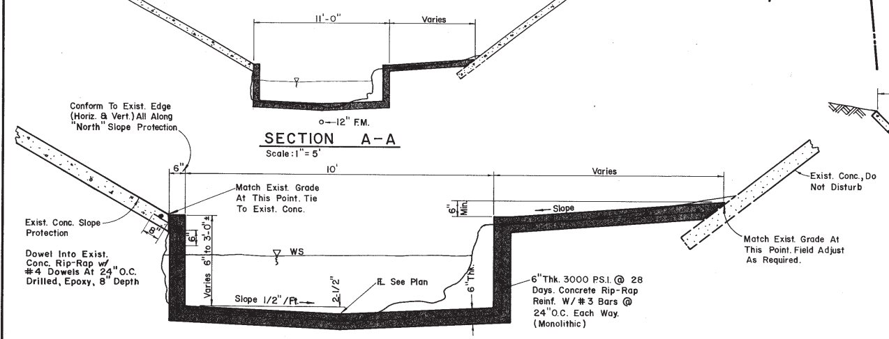
TYPICAL CHANNEL SECTION DETAIL Scale: 1/2" = 1'-0"
