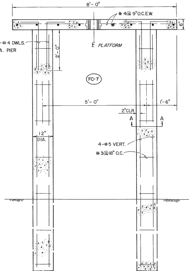
REINFORCEMENT DETAIL
