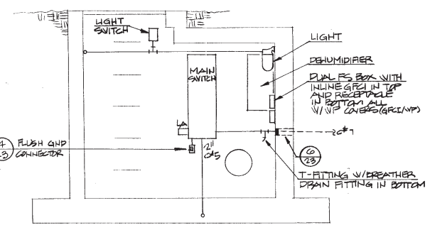
3 SECTION B SCALE 3/8" = 1'-0"
