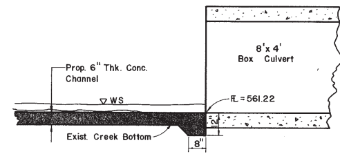
SECTION X-X DETAIL AT BOX CULVERT Scale: 3/8" = 1'
