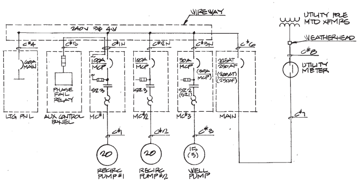
4 ONE LINE DIAGRAM
