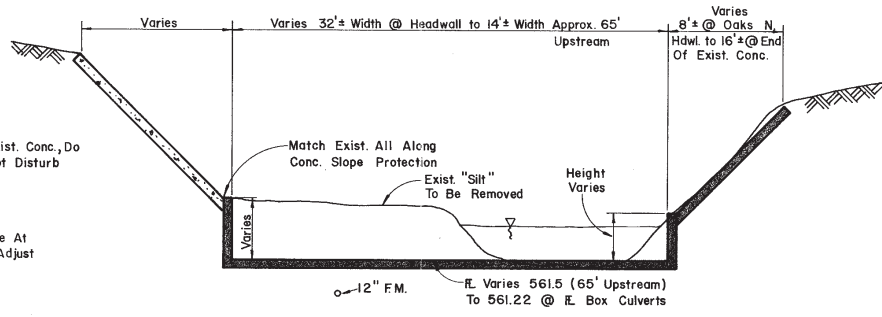
SECTION B-B No Scale
