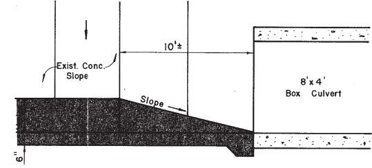
SECTION Y-Y No Scale
