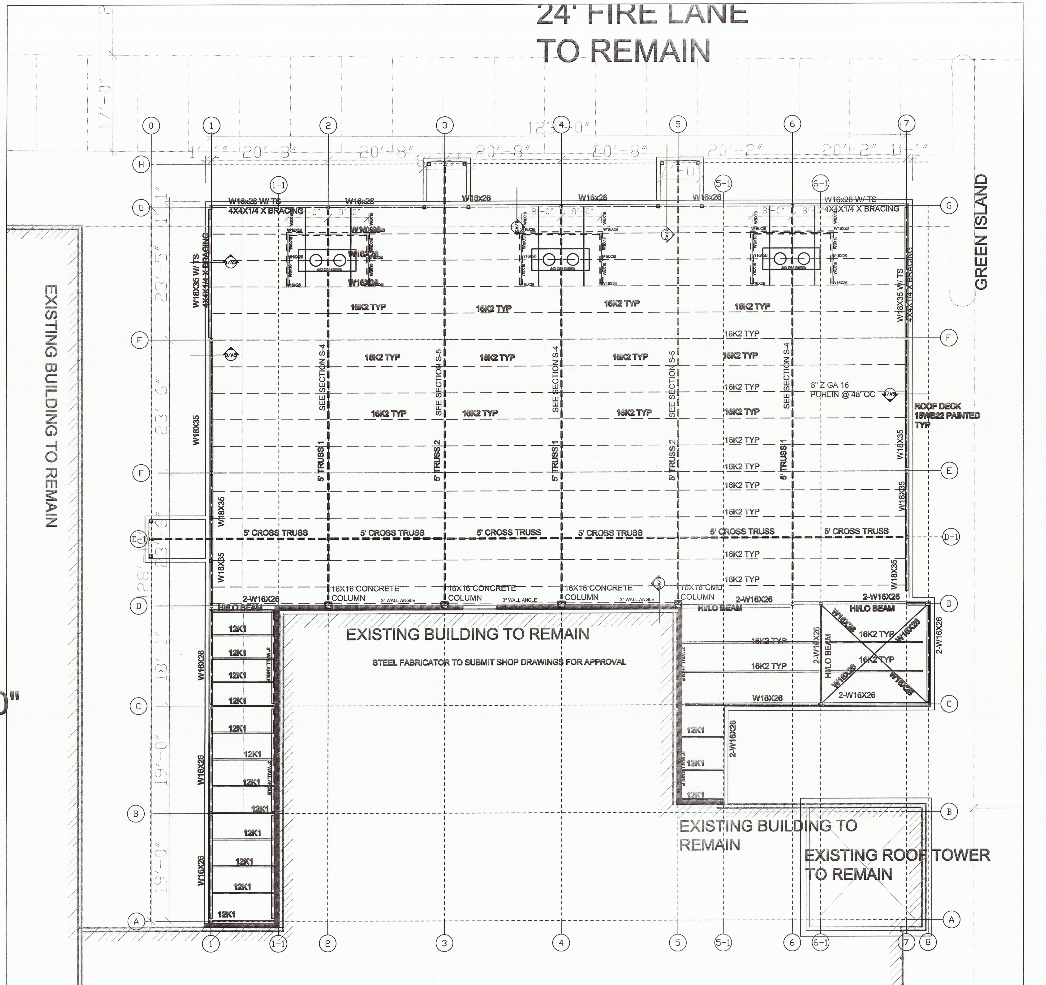
ROOF FRAMING S: 1/8"=1'-0"
