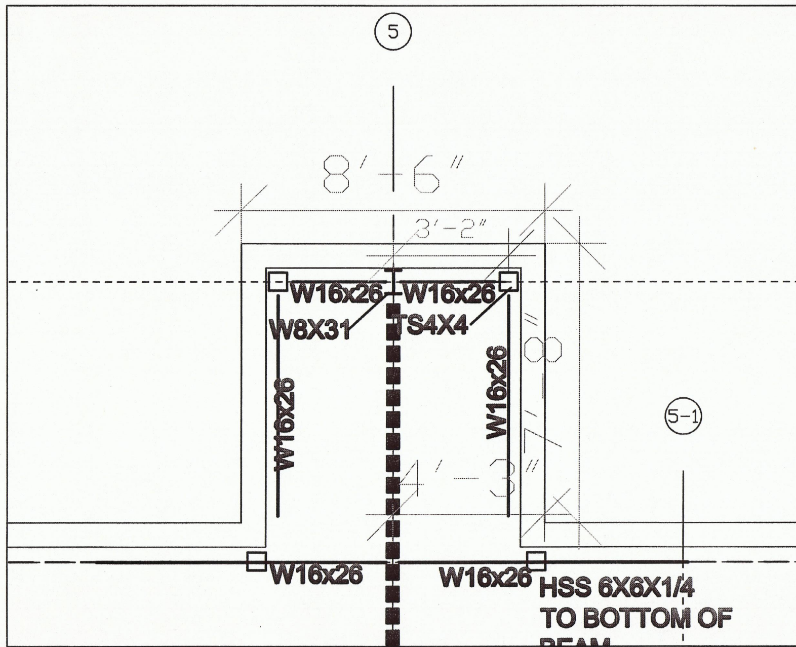
PANEL POCKET S: 3/8"=1'-0"
