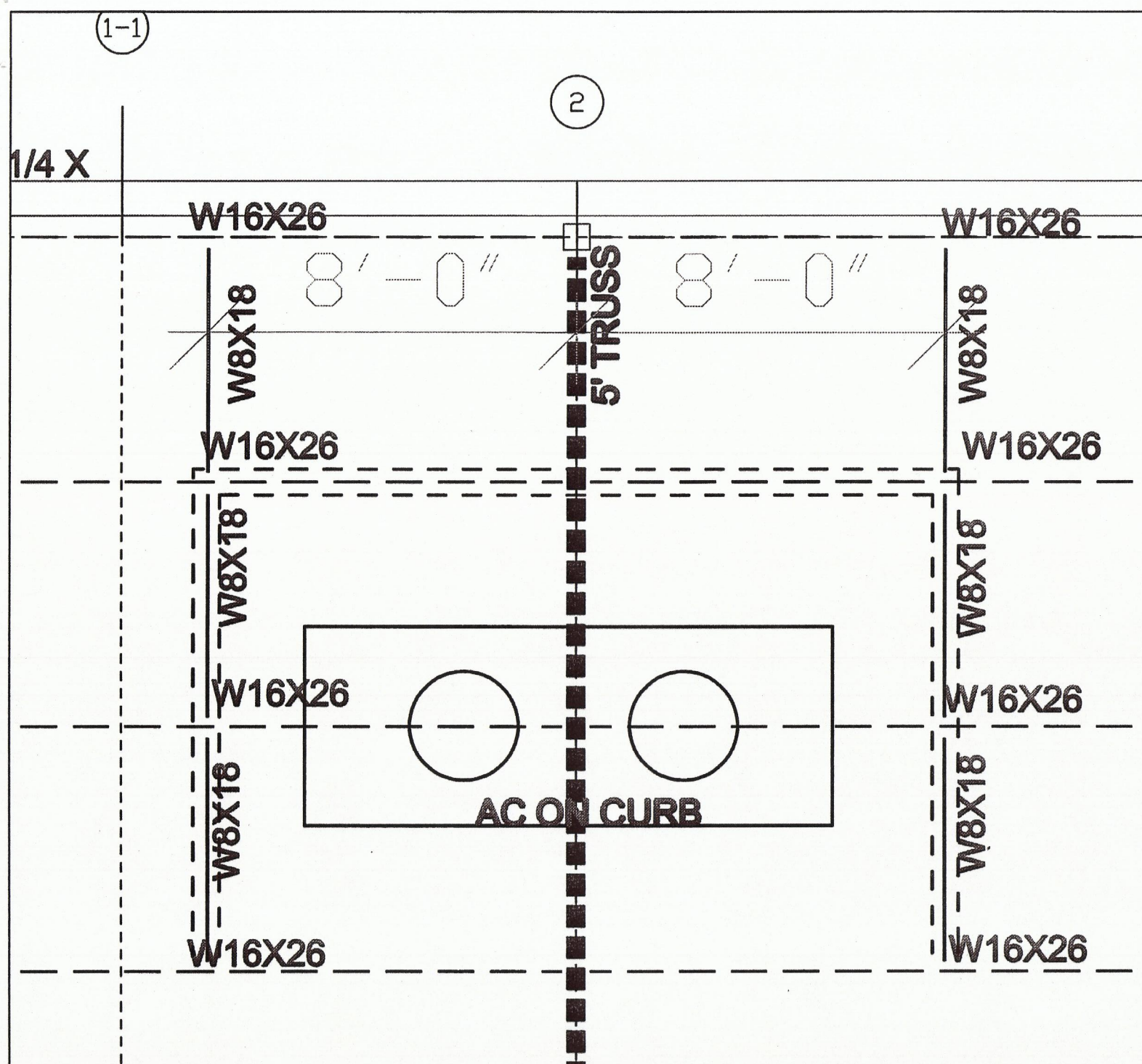
RTU SCREENS: 3/8"=1'-0"
