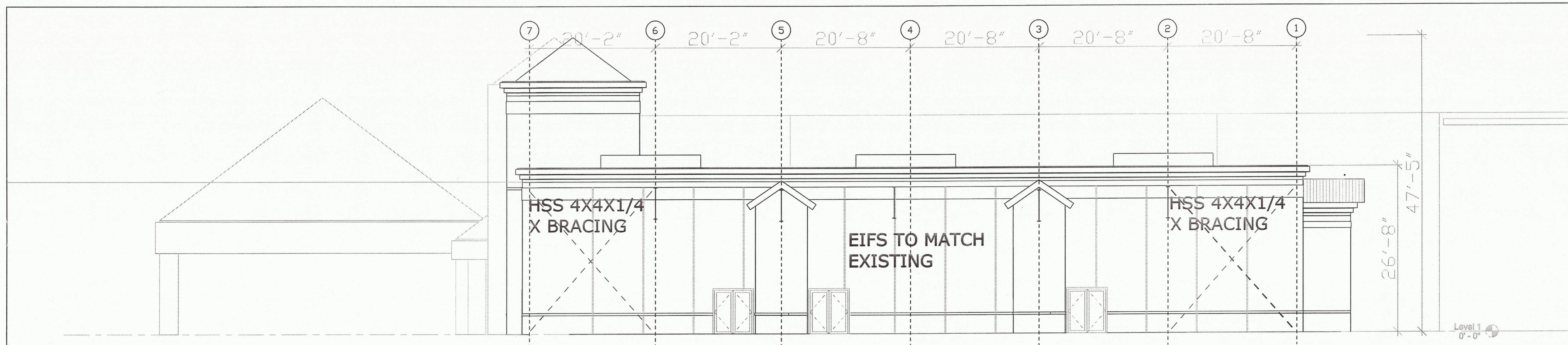
NORTH ELEVATION S: 1/8"=1'-0"
