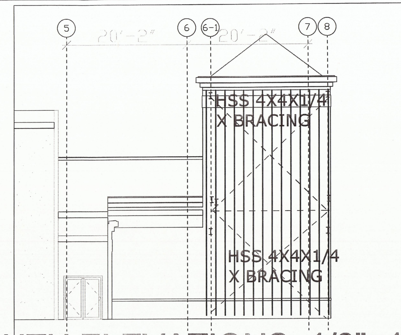
SOUTH ELEVATIONS: 1/8"=1'-0"
