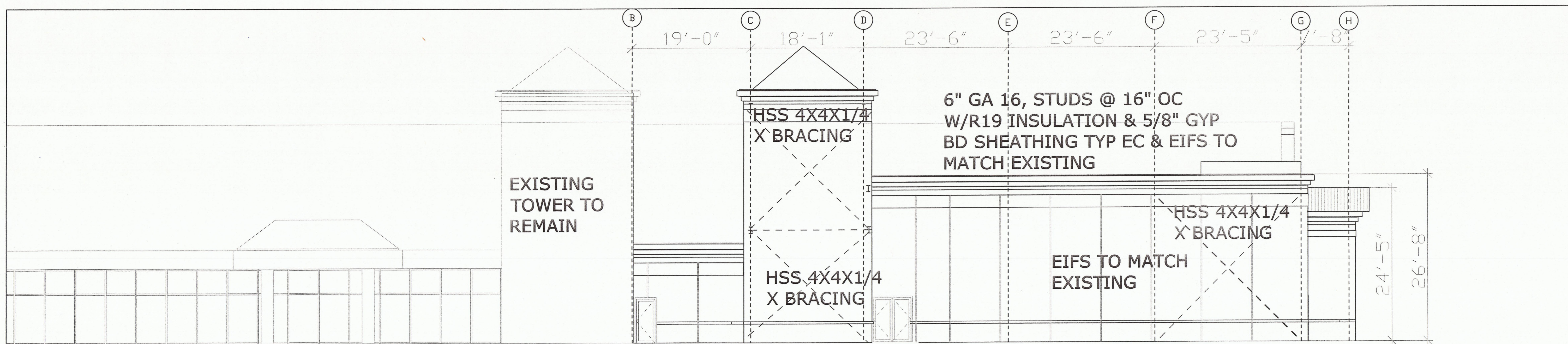
EAST ELEVATIONS: 1/8"=1'-0"
