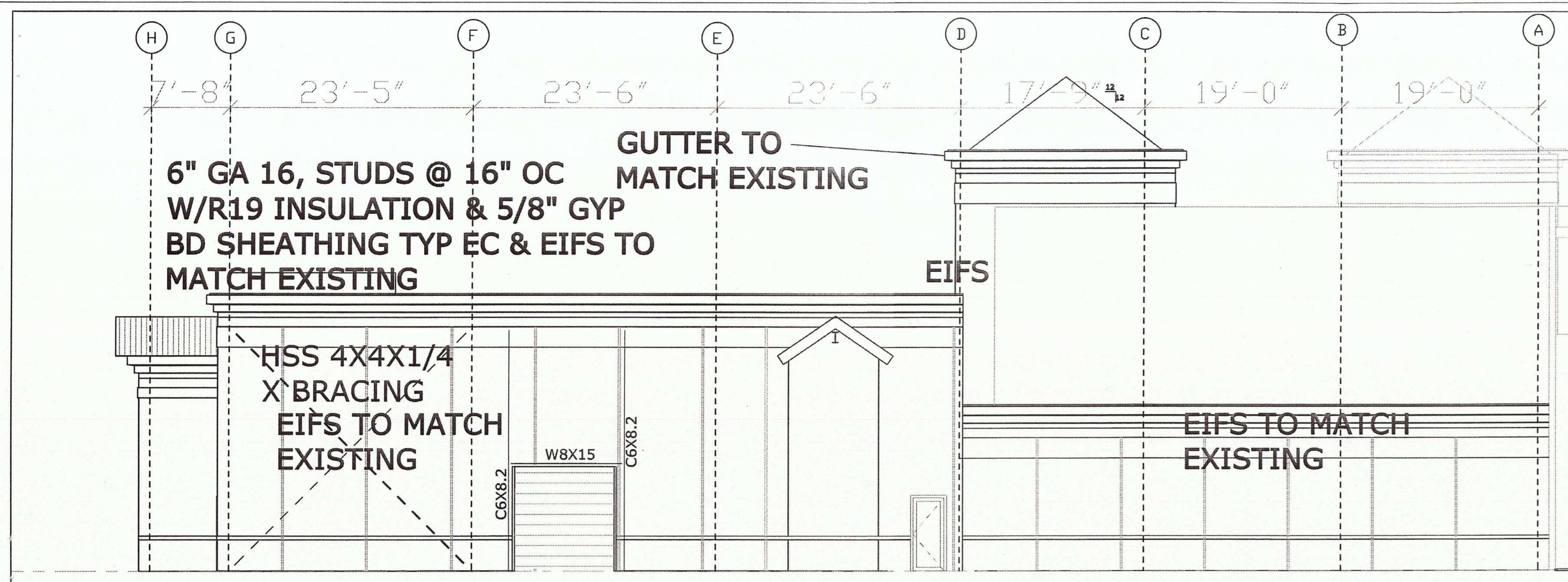
WEST ELEVATIONS: 1/8"=1'-0"
