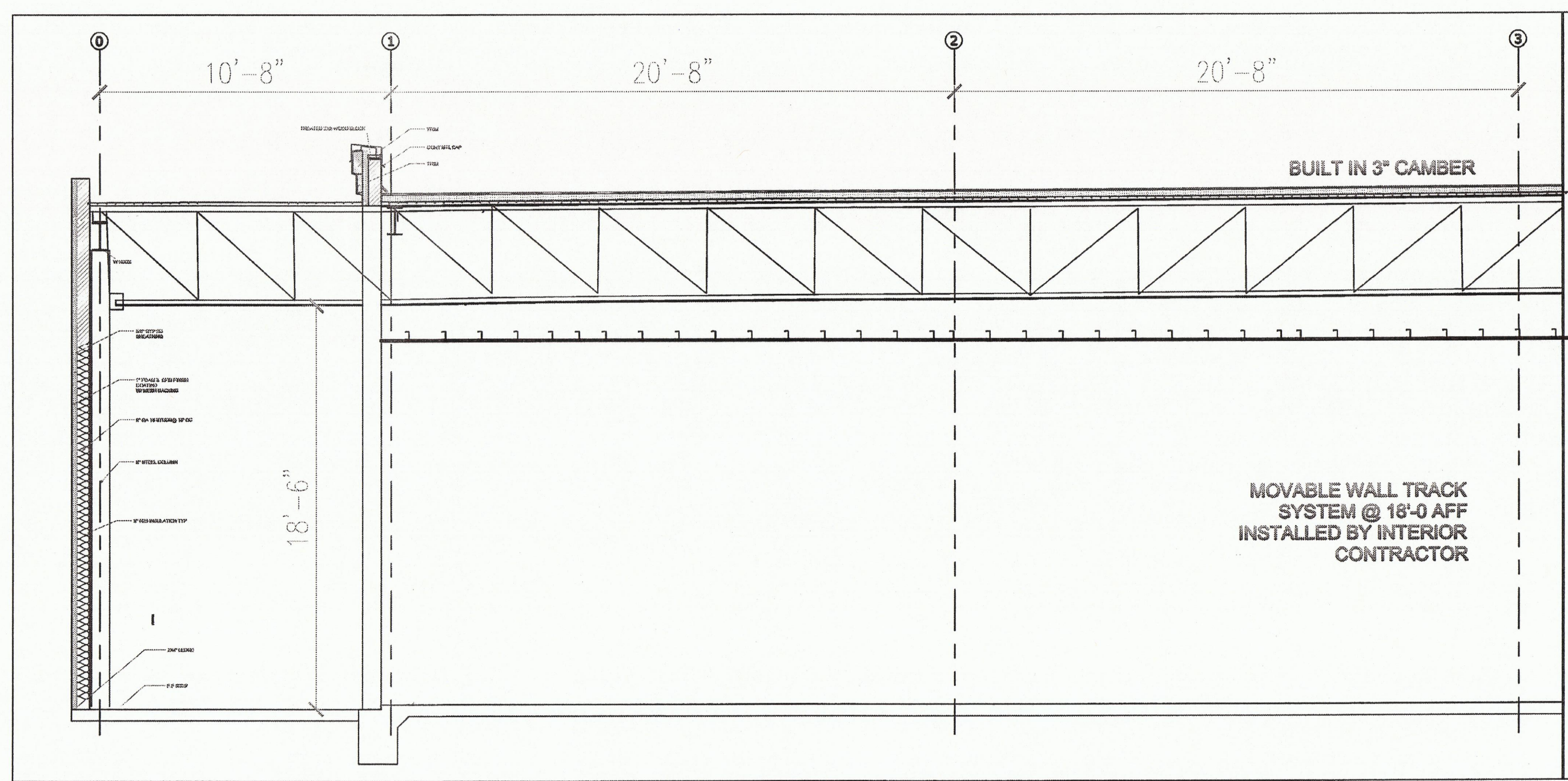
5' CROSS TRUSS CONFIG. S: 1/4"=1'-0"
