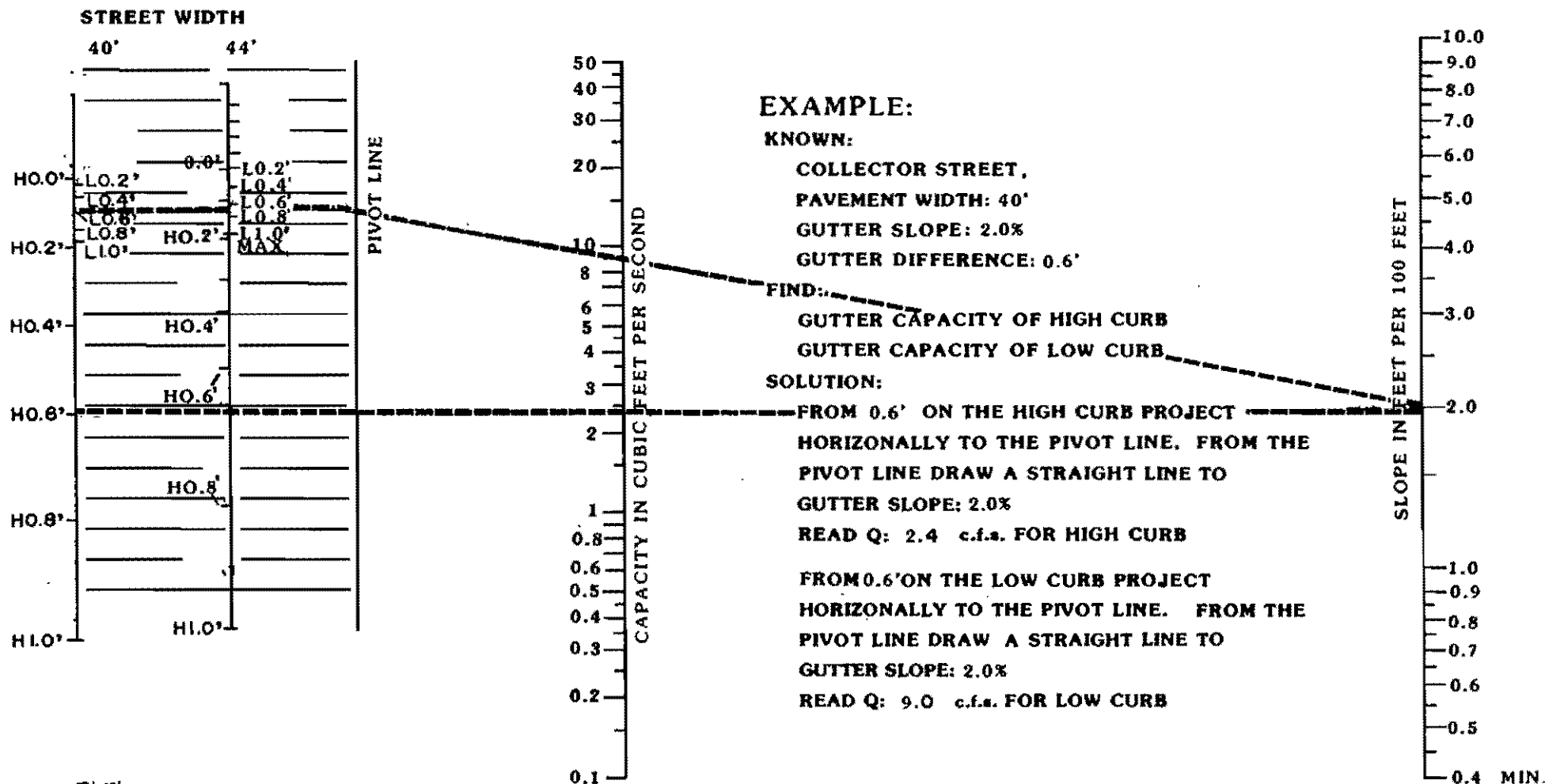
CAPACITY OF PARABOLIC GUTTERS (40' & 44' STREET WIDTHS)
