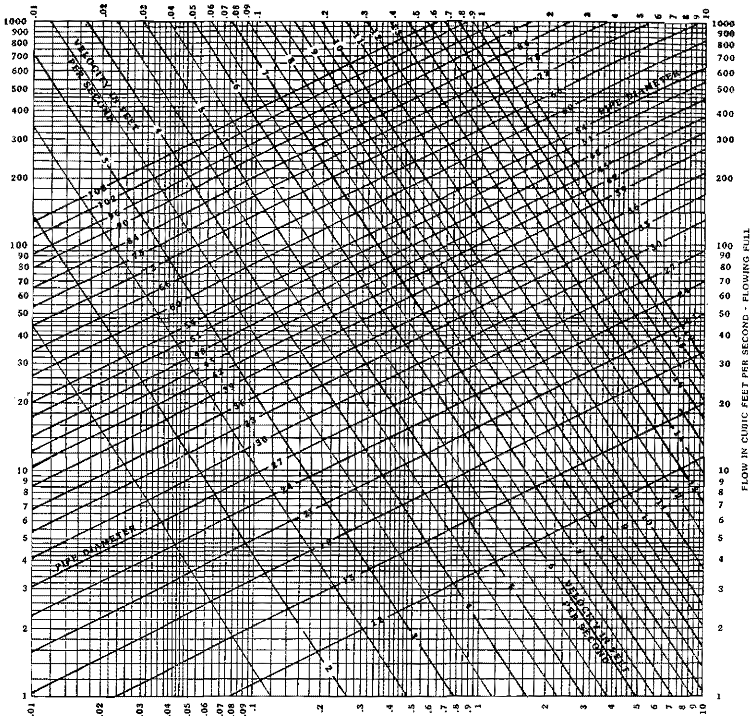
SLOPE OF PIPE IN FEET PER 100 FEET CAPACITY OF CIRCULAR PIPES FLOWING FULL FIGURE 22
