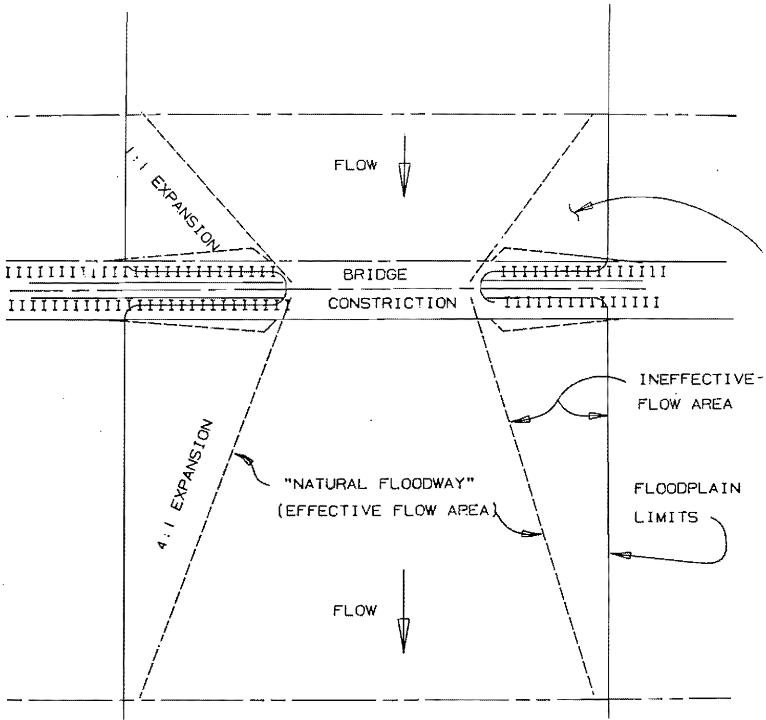
FIGURE 25. "NATURAL FLOODWAY" EXAMPLE
