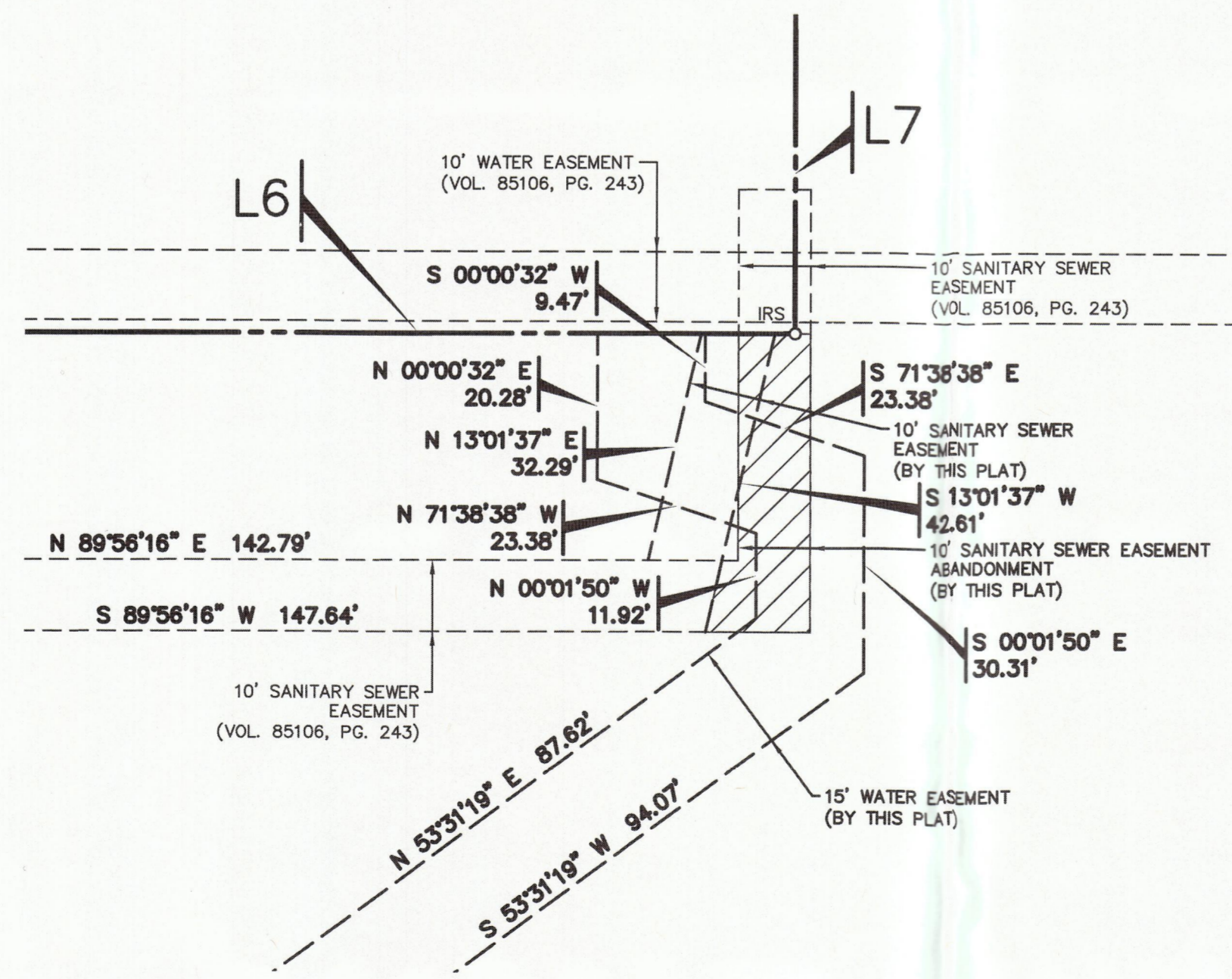
1 DETAIL SCALE 1"=20'
